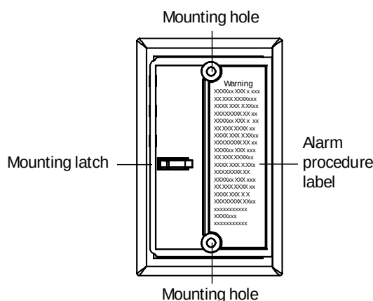
Figure 6: Horizontal mounting
