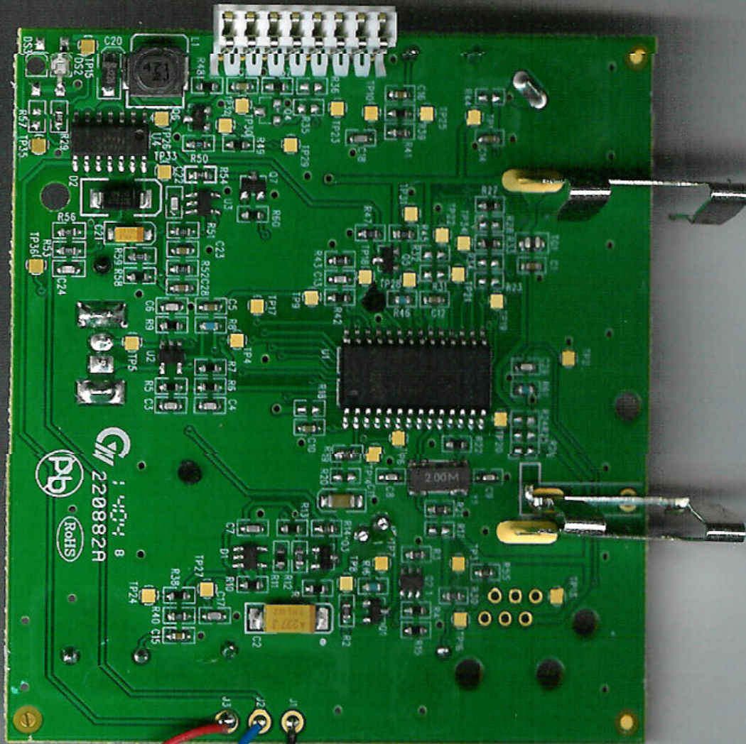
Smoke Detector PWB
