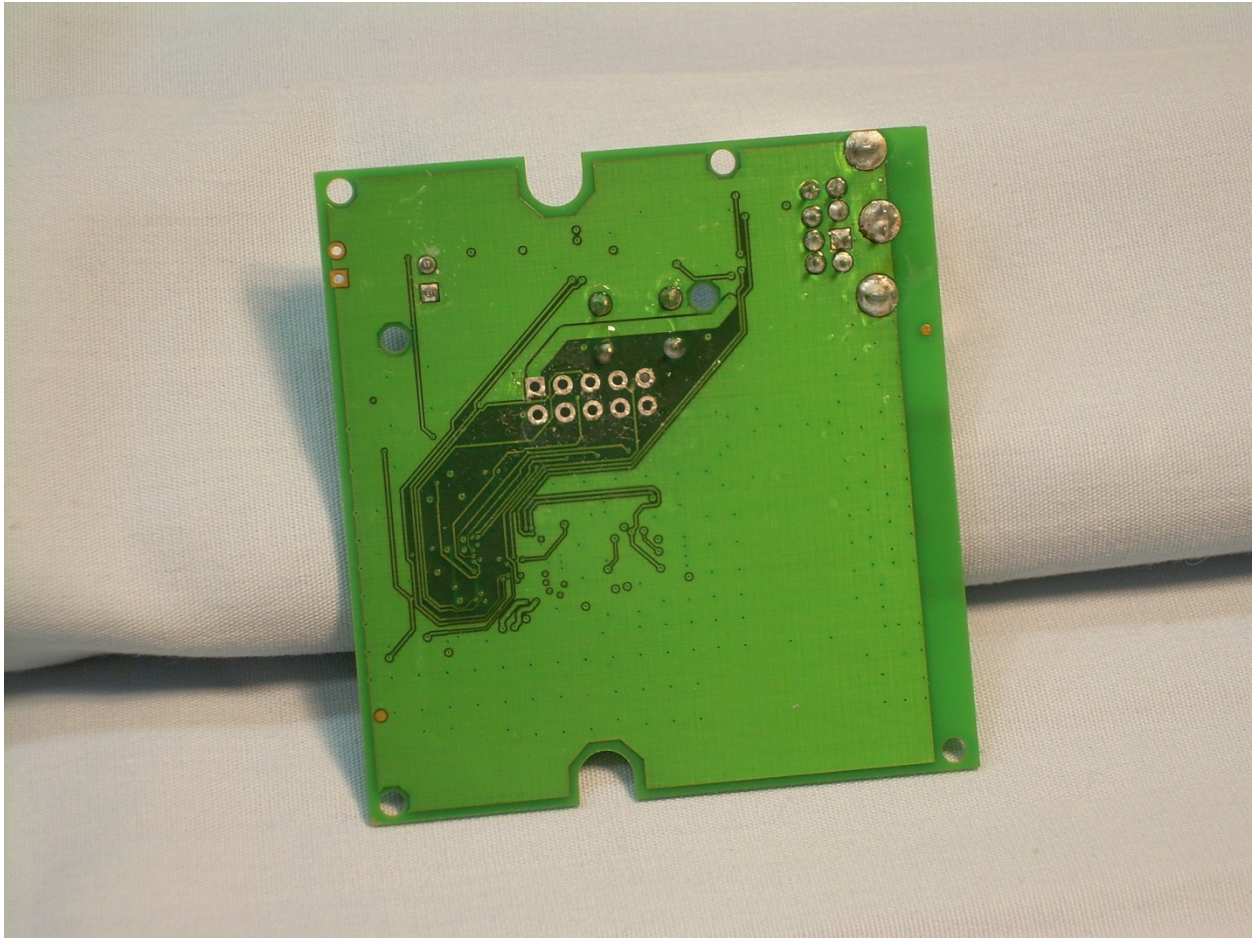
View of the Bottom Side of the PCB
