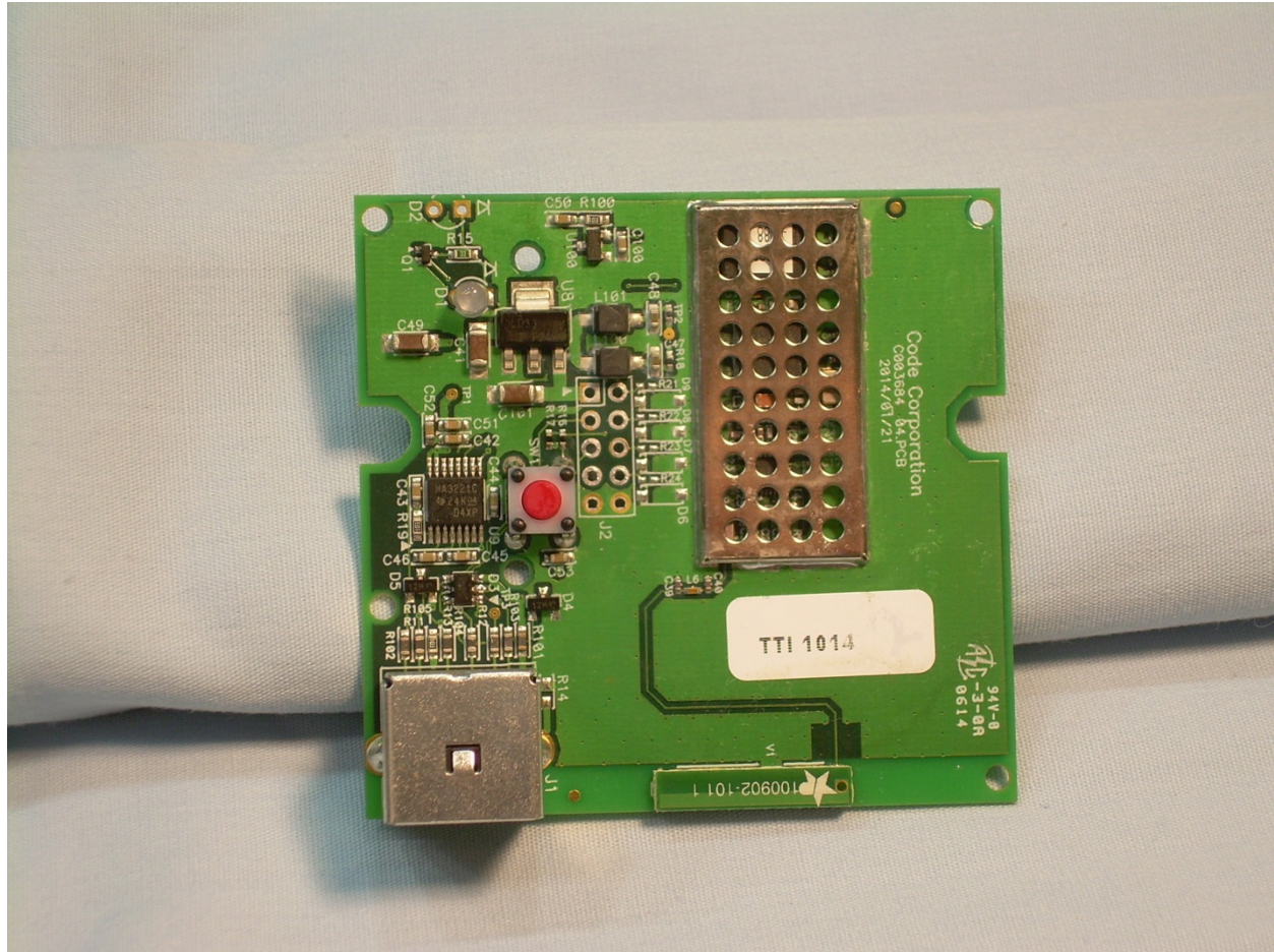
View of the Top Side of the PCB with RF Shield In Place
