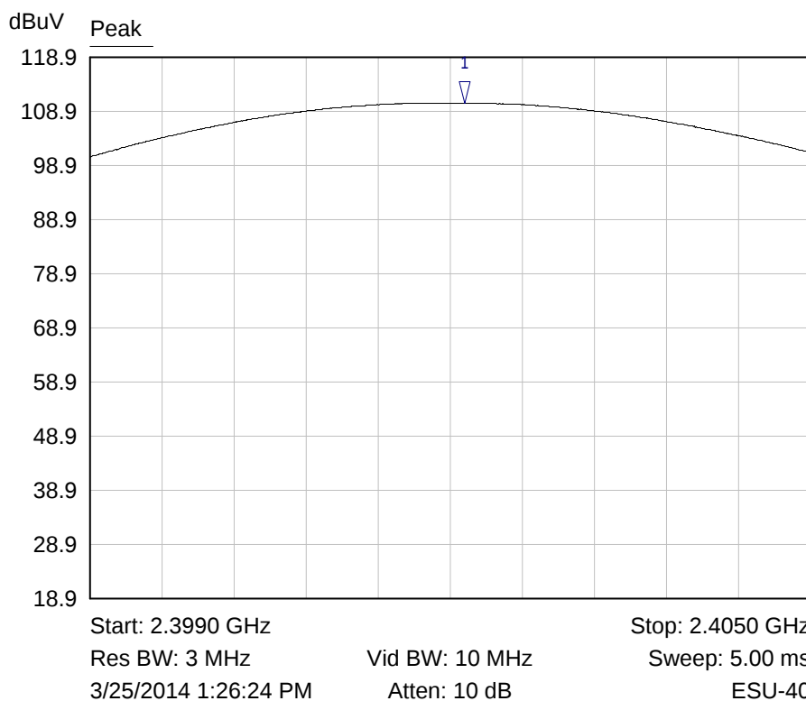
Lowest Channel Fundamental Field Strength
