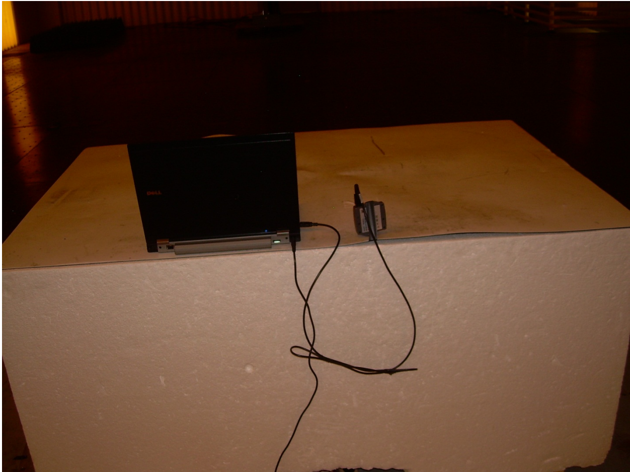
Photograph 4 – Back View Radiated Disturbance Configuration – Vertical
