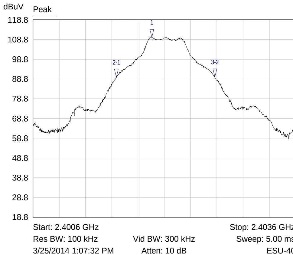
Lowest Channel 20 dB Bandwidth
