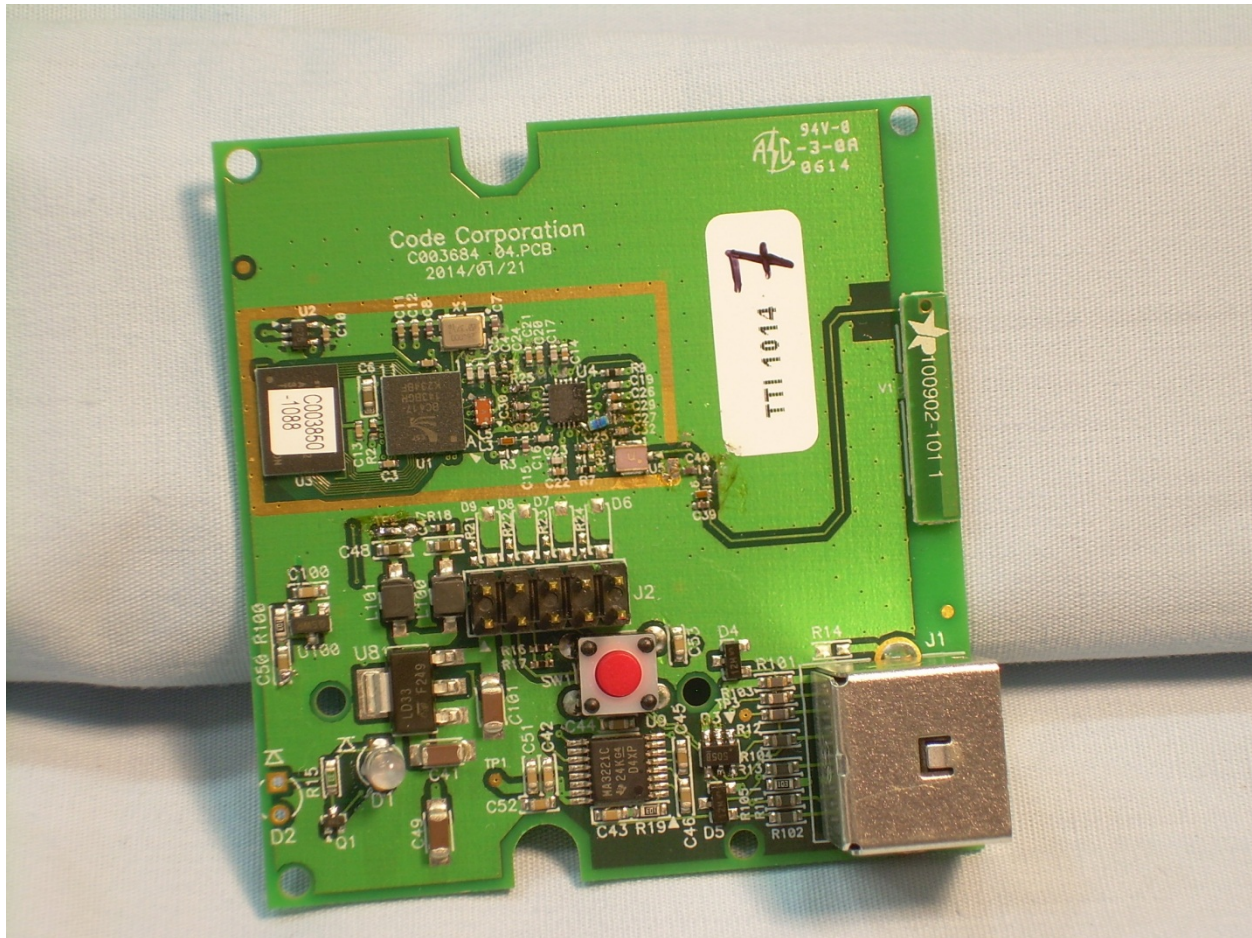
Photograph 11 – View of the Top Side of the PCB with RF Shield Removed
