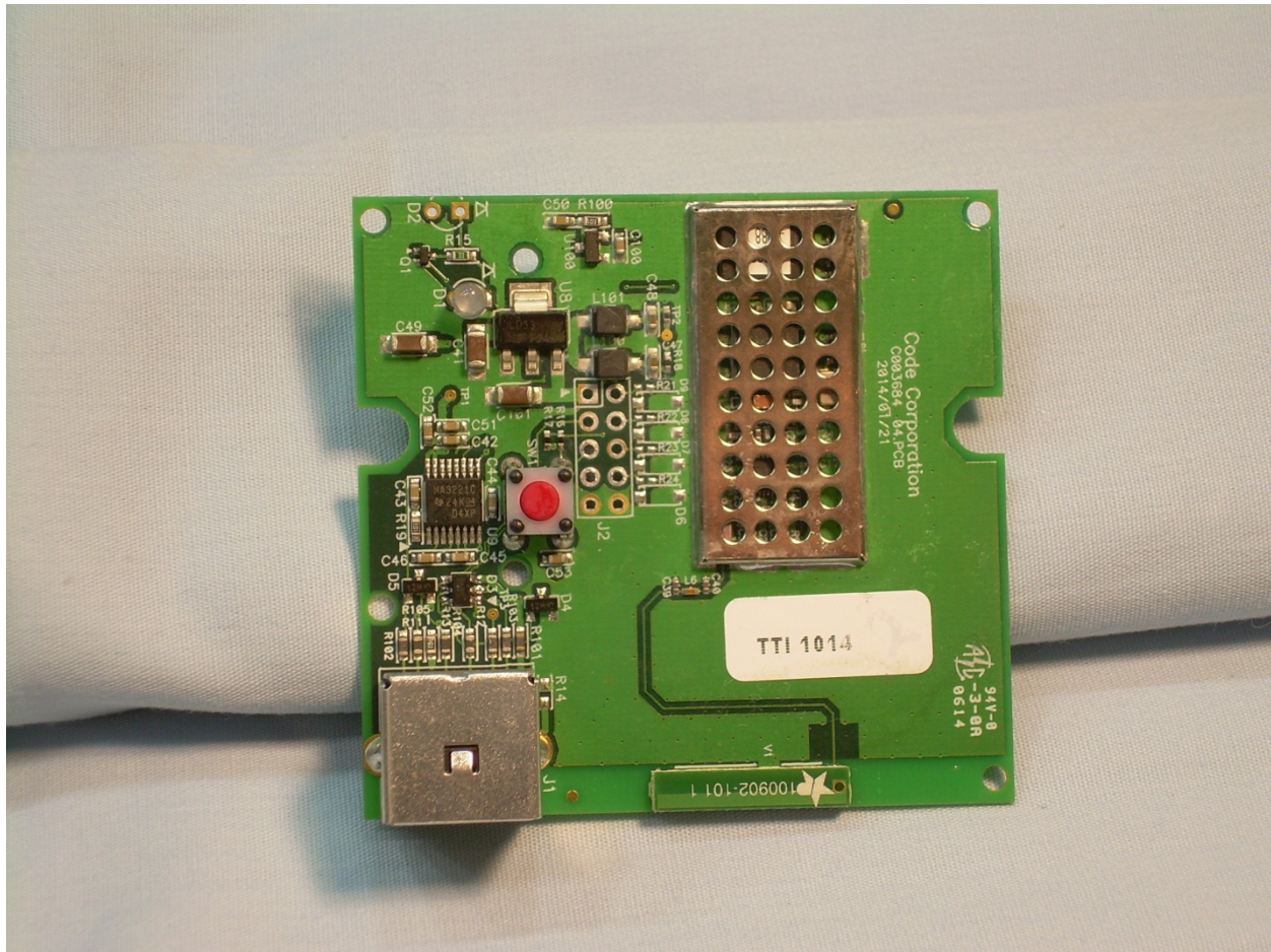
Photograph 10 – View of the Top Side of the PCB with RF Shield In Place
