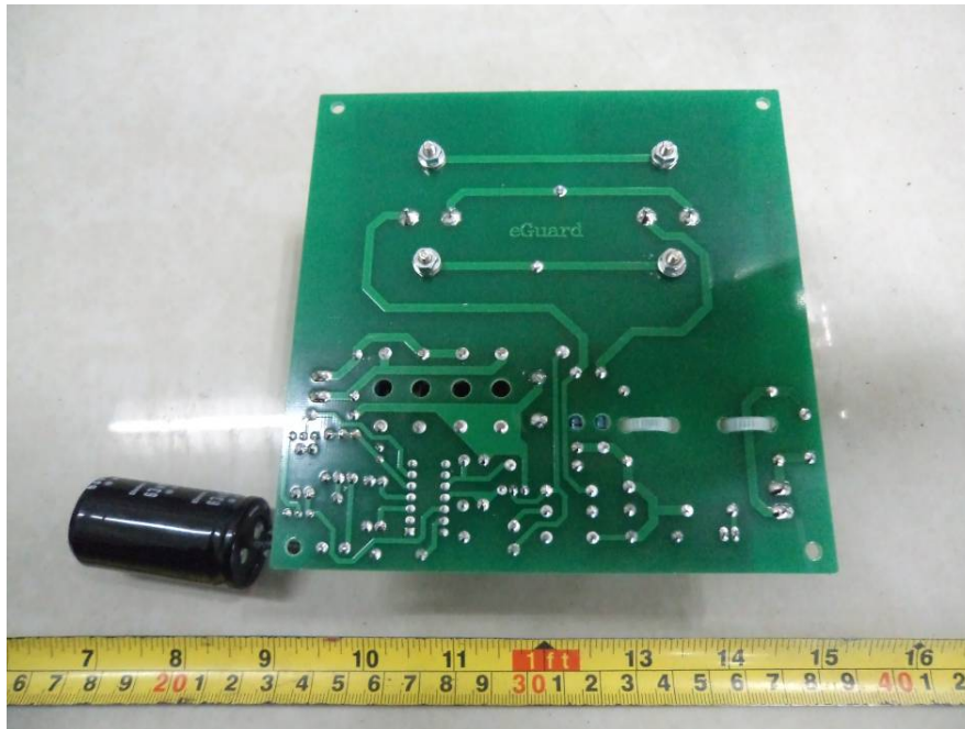
EUT – Main Board Bottom View Shielding off(DC Power)
