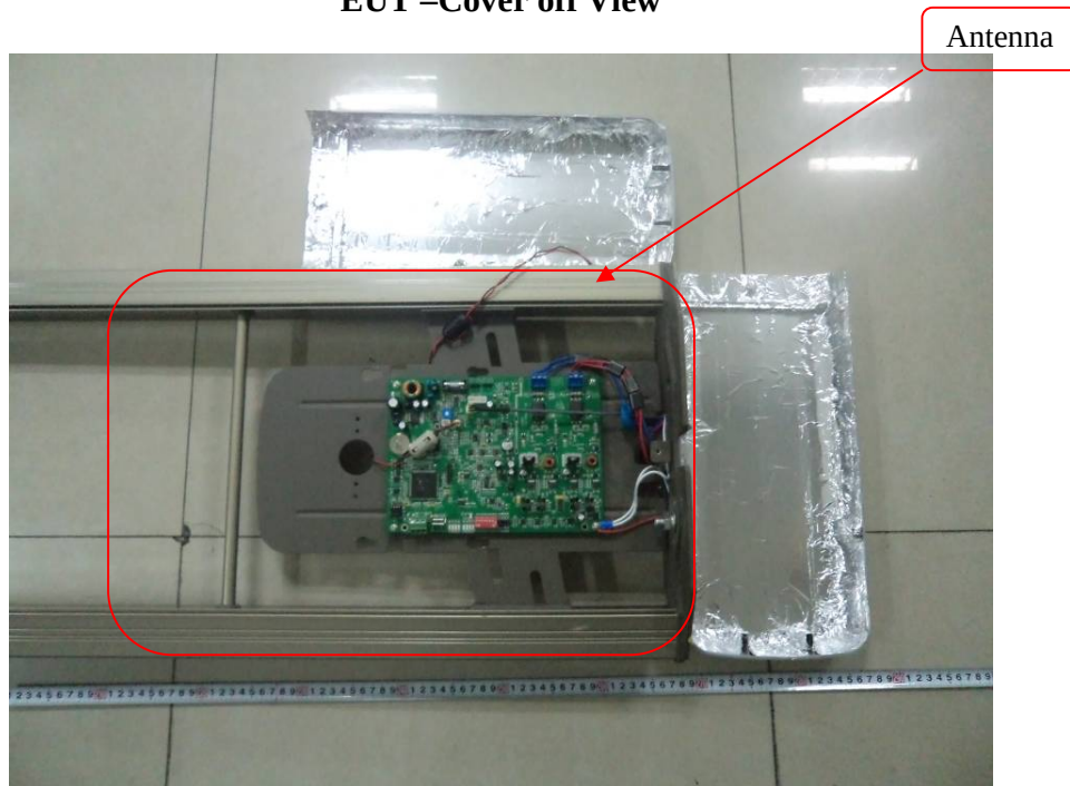
EUT –Cover off View
