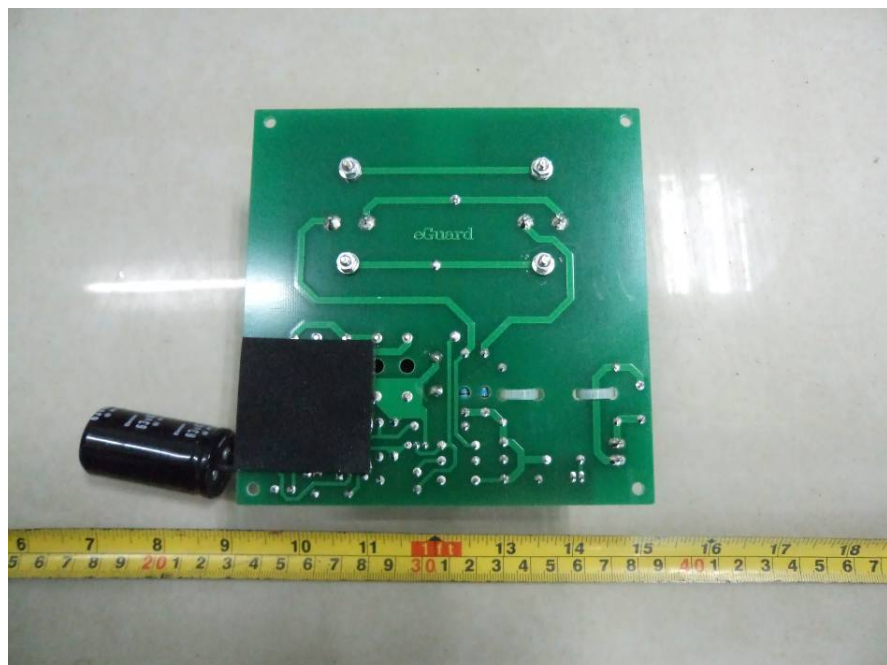
EUT – Main Board Bottom View (DC Power)
