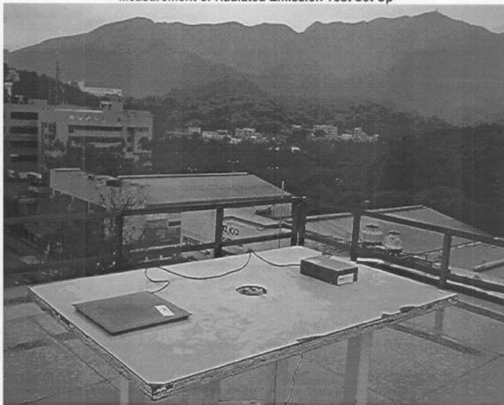
Measurement of Radiated Emission Test Set Up
