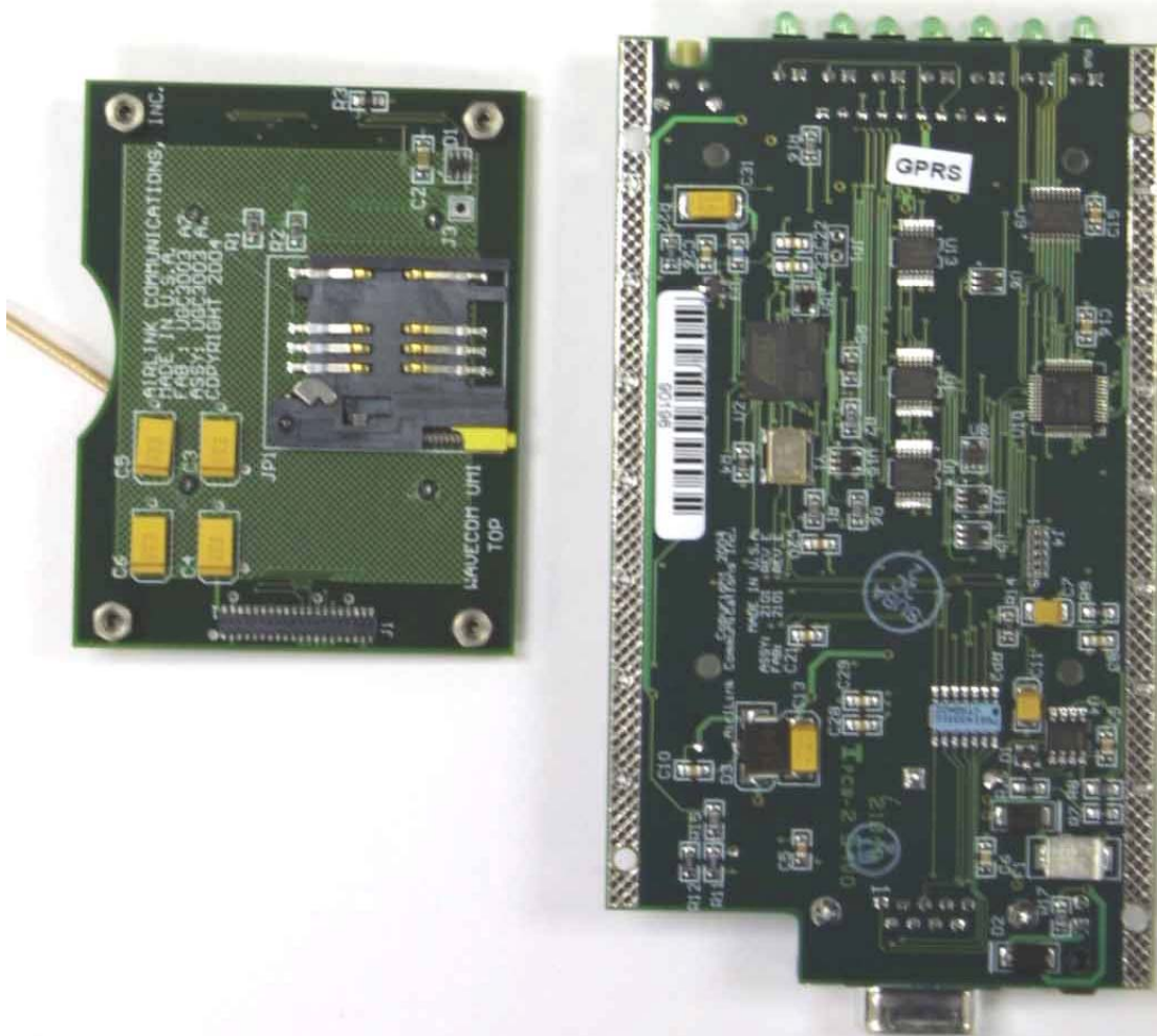
EUT – Internal Bottom view
