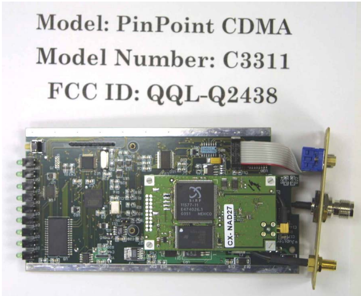
EUT – Internal Top view
