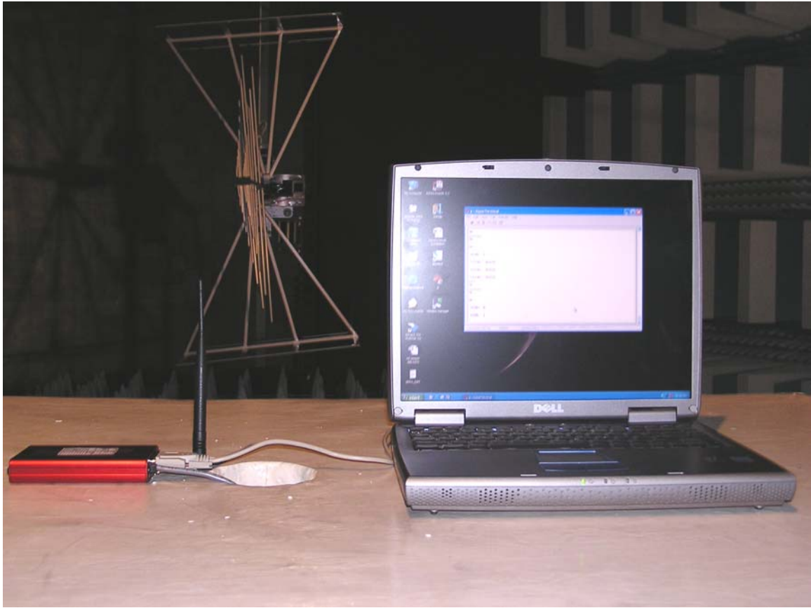
Test setup – Radiated Emissions Redwing
