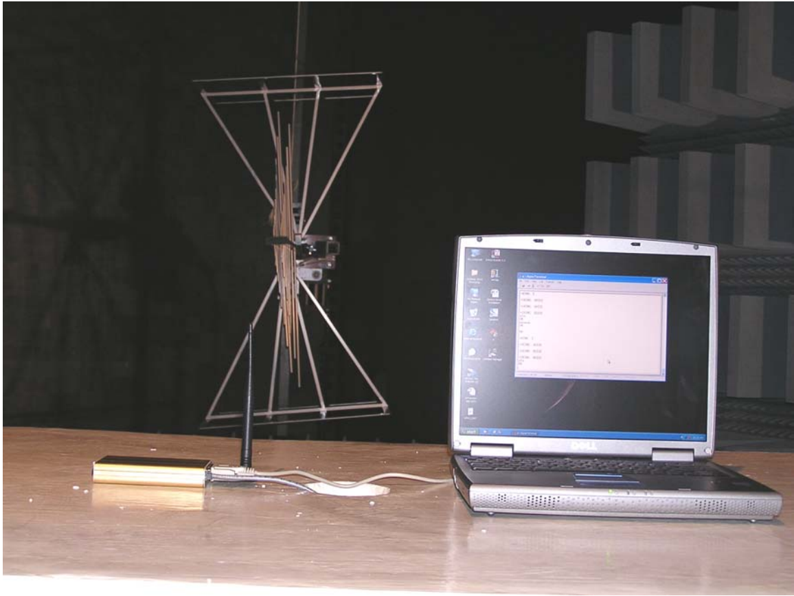
Test setup – Radiated Emissions Raven
