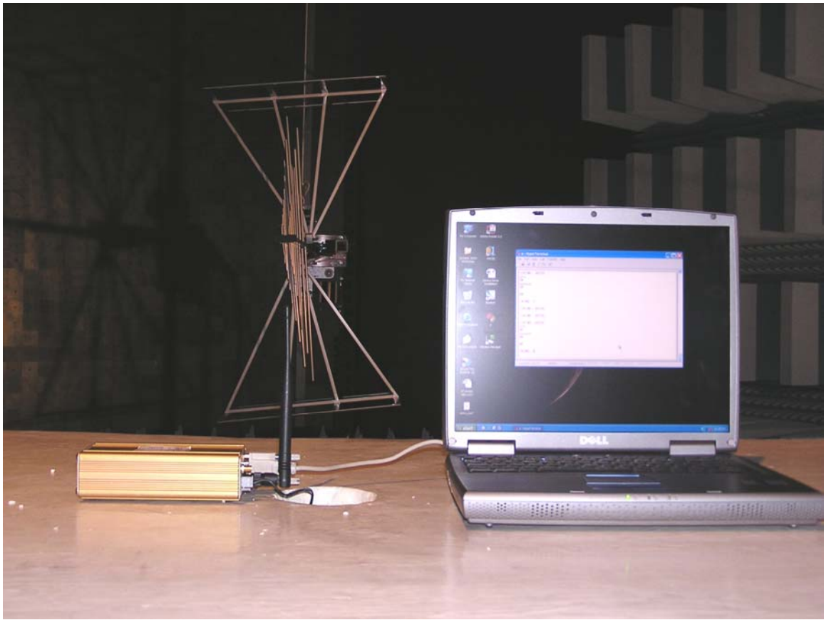
Test setup – Radiated Emissions Pinpoint
