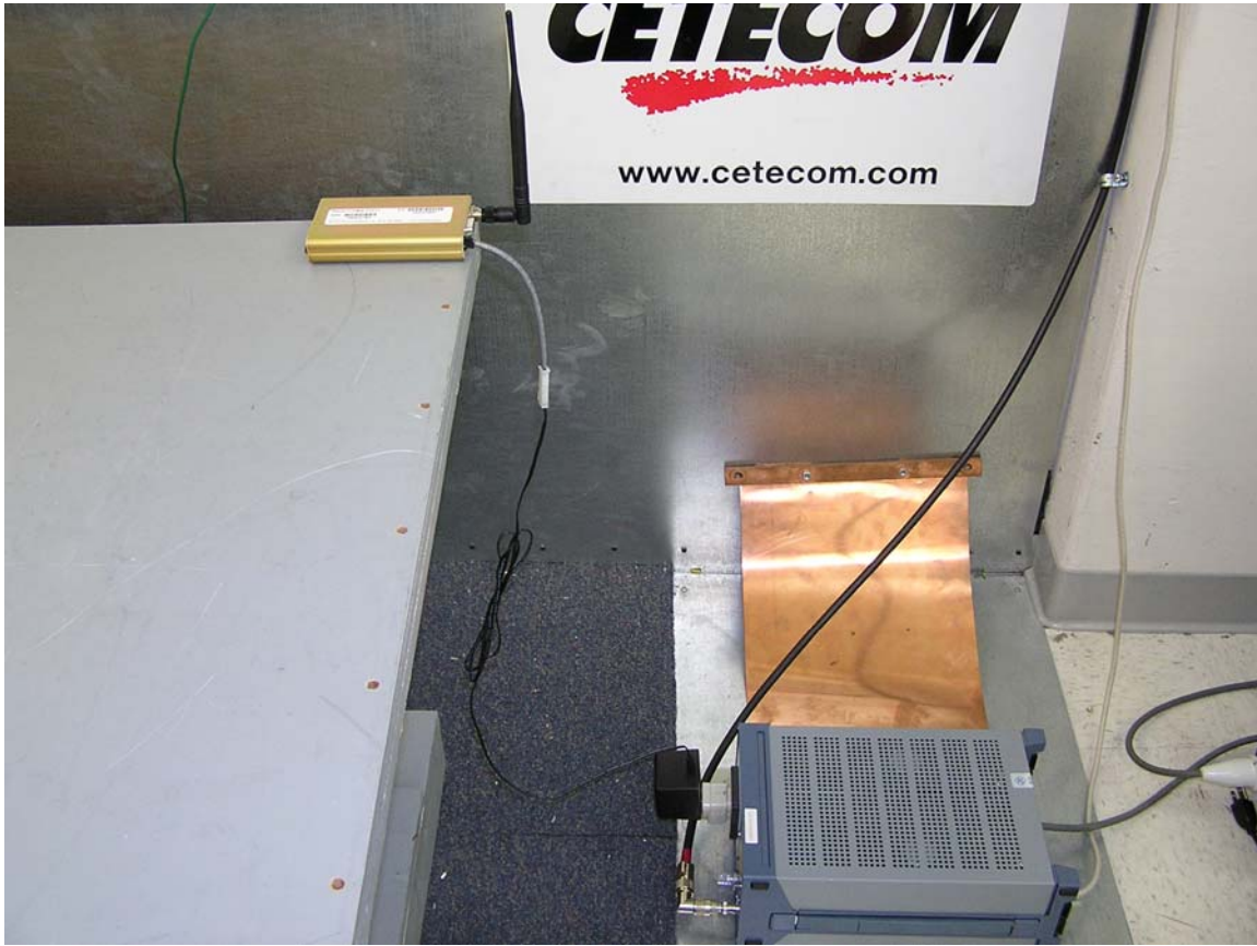
Test setup – AC Line Conducted Emissions Raven
