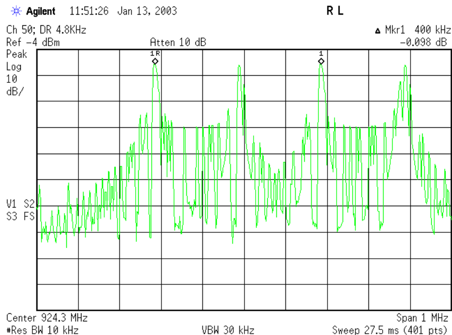
Plot #2 Showing carrier frequency separation (hopping enabled)
