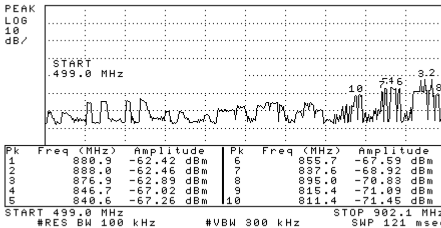
Plot #21 Showing Spurious RF Conducted Emissions 500-902MHz (data rate 4.8KHz)
