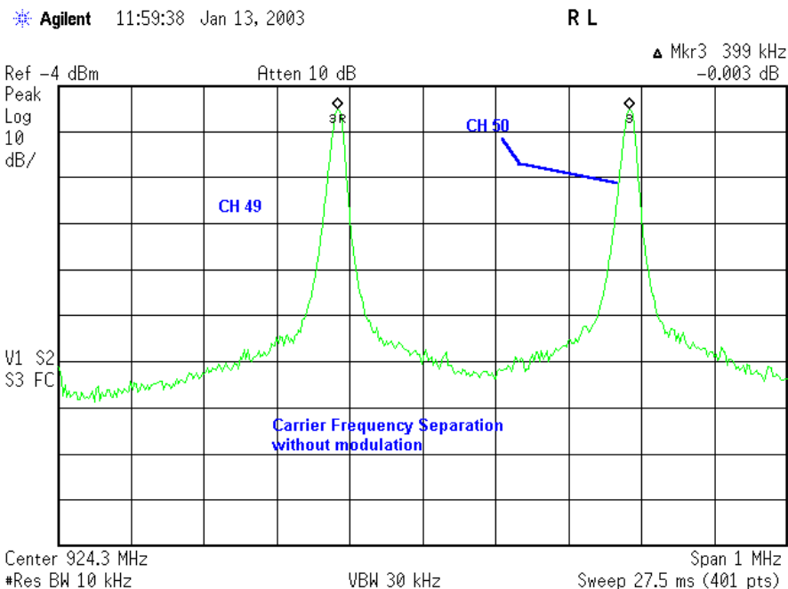
Plot #1 Showing carrier frequency separation (hopping disabled)
