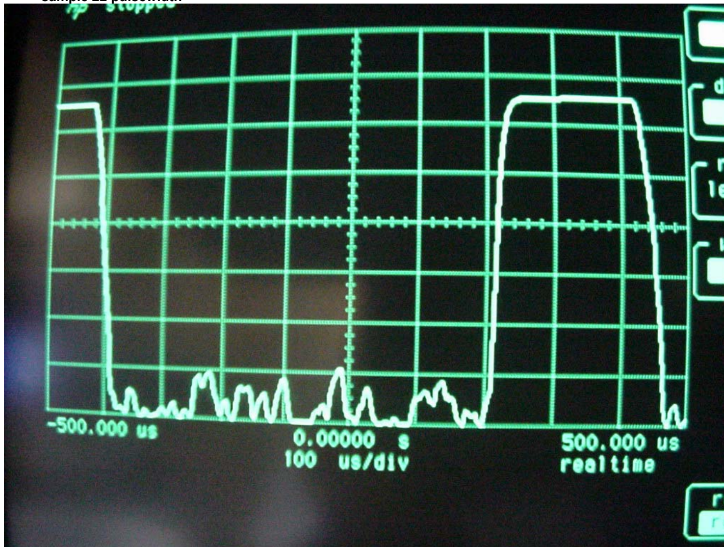
sample 22 pulsewidth
