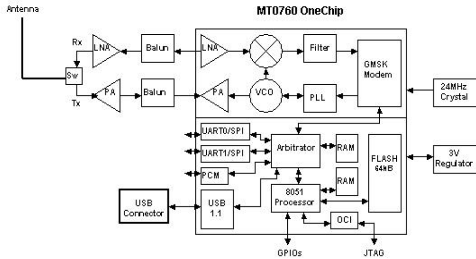
Block Diagram MT0760-UD1P
