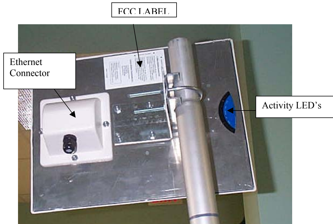
TR 3315 Rear View
