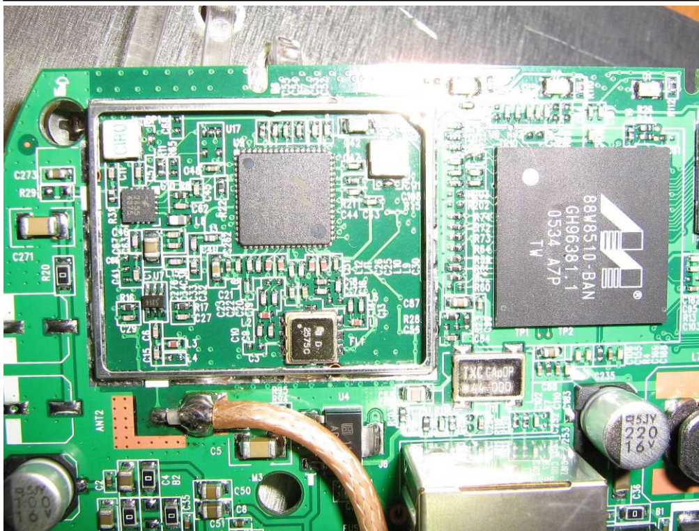
Radio Module with RF shield removed.
