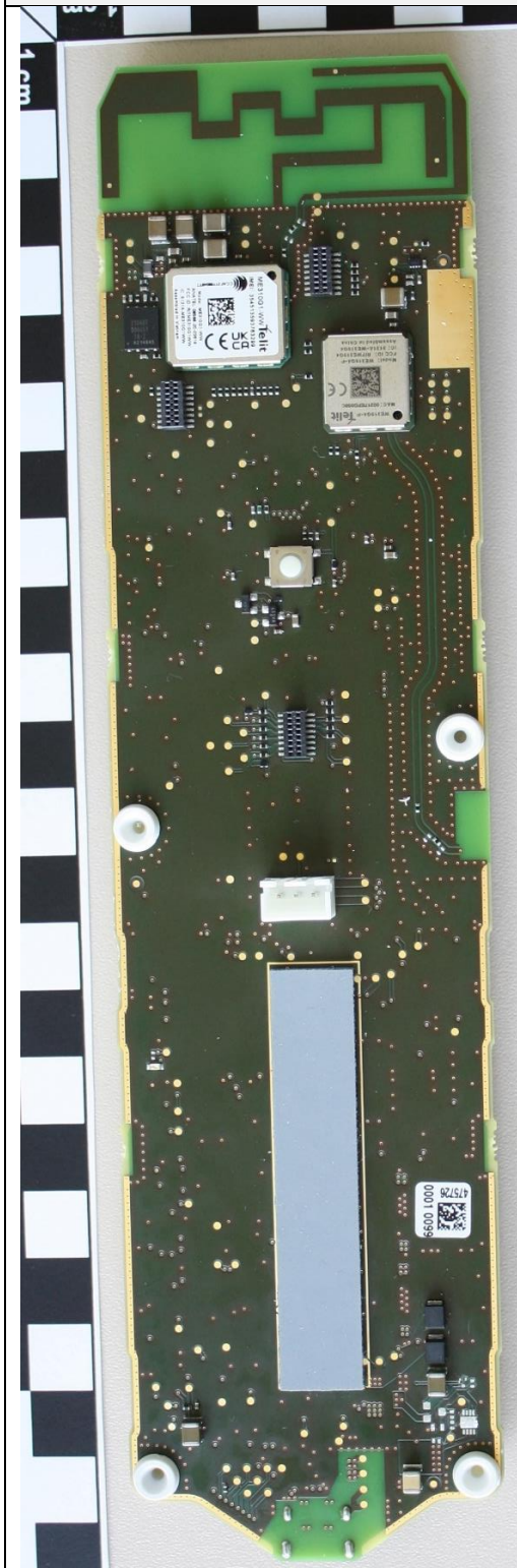
MainPCB-LP1-bottom-shields-installed
