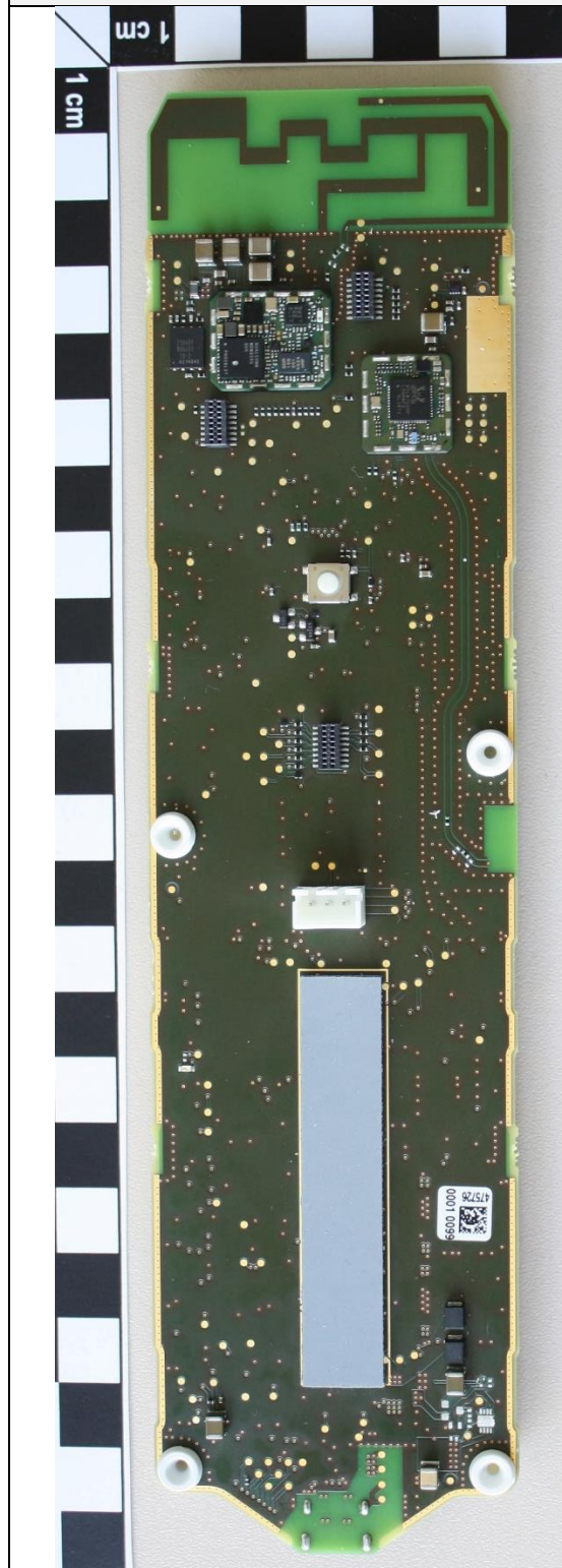
MainPCB-LP1-top-shields-removed
