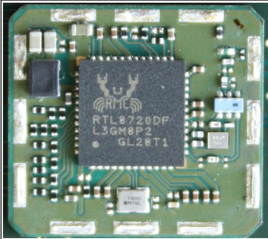
IEEE 802.11 Radio module: we310g4 PCB shields removed
