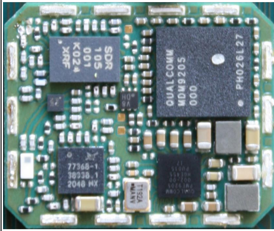
LTE Radio module: me310g1 PCB shields removed
