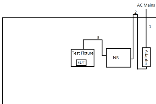
Test Setup Diagram - Radiated Test (WE310G4-I)
