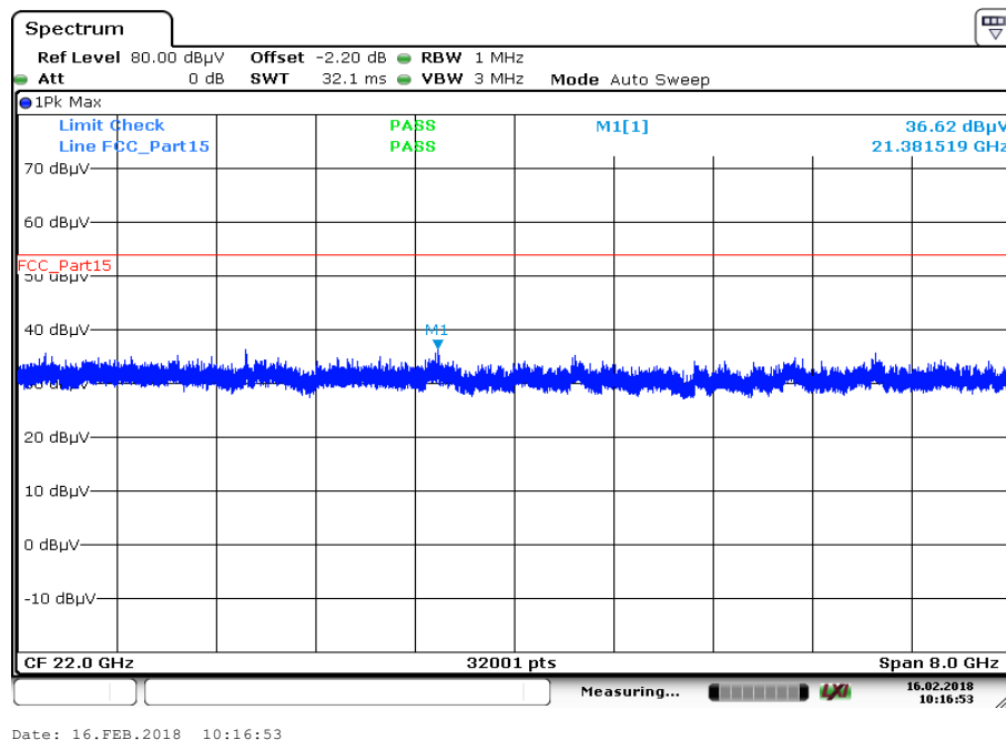
Plot 24: 18 GHz to 26 GHz, TX mode, 2480 MHz, vertical &amp; horizontal polarization, 2 Msps, external antenna
