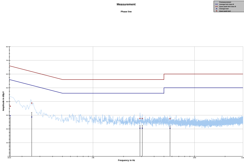
Plot 3: 150 kHz to 30 MHz, phase line, internal antenna
