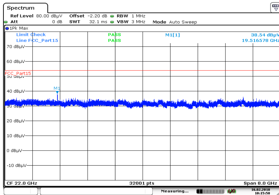
Plot 22: 18 GHz to 26 GHz, TX mode, 2440 MHz, vertical &amp; horizontal polarization, 2 Msps, external antenna
