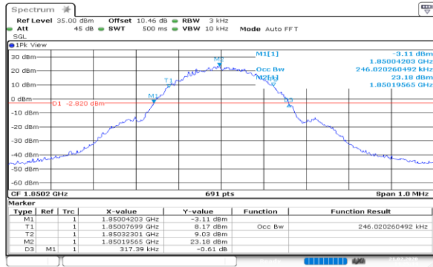
GPRS_1900_Lower_26BW and 99%
