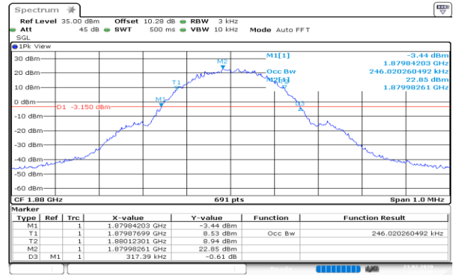
GPRS_1900_Middle_26BW and 99%
