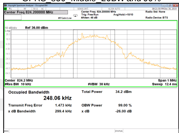
EGPRS(8PSK) 850 Lower 26BW and 99%
