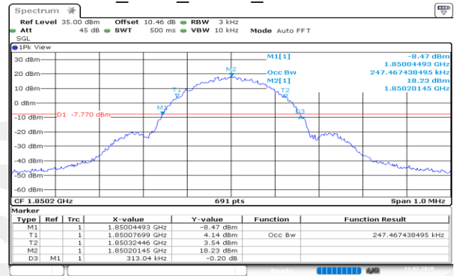
EGPRS(8PSK)_1900_Lower_26BW and 99%
