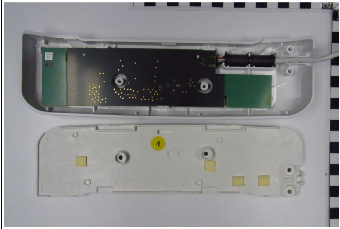
Interior view, PCB bottom view
