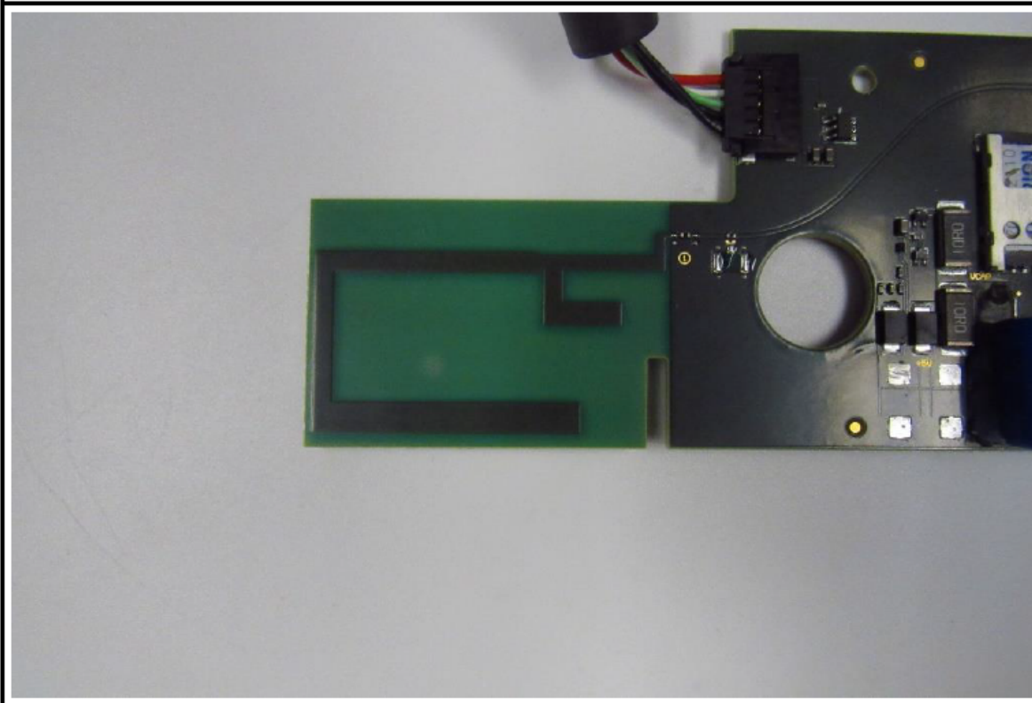
Antenna A view
