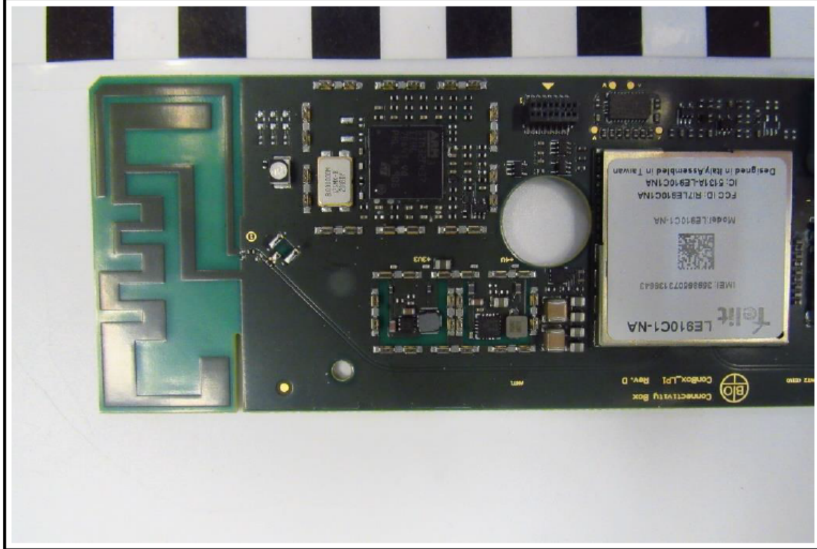
Antenna B view, no shielding
