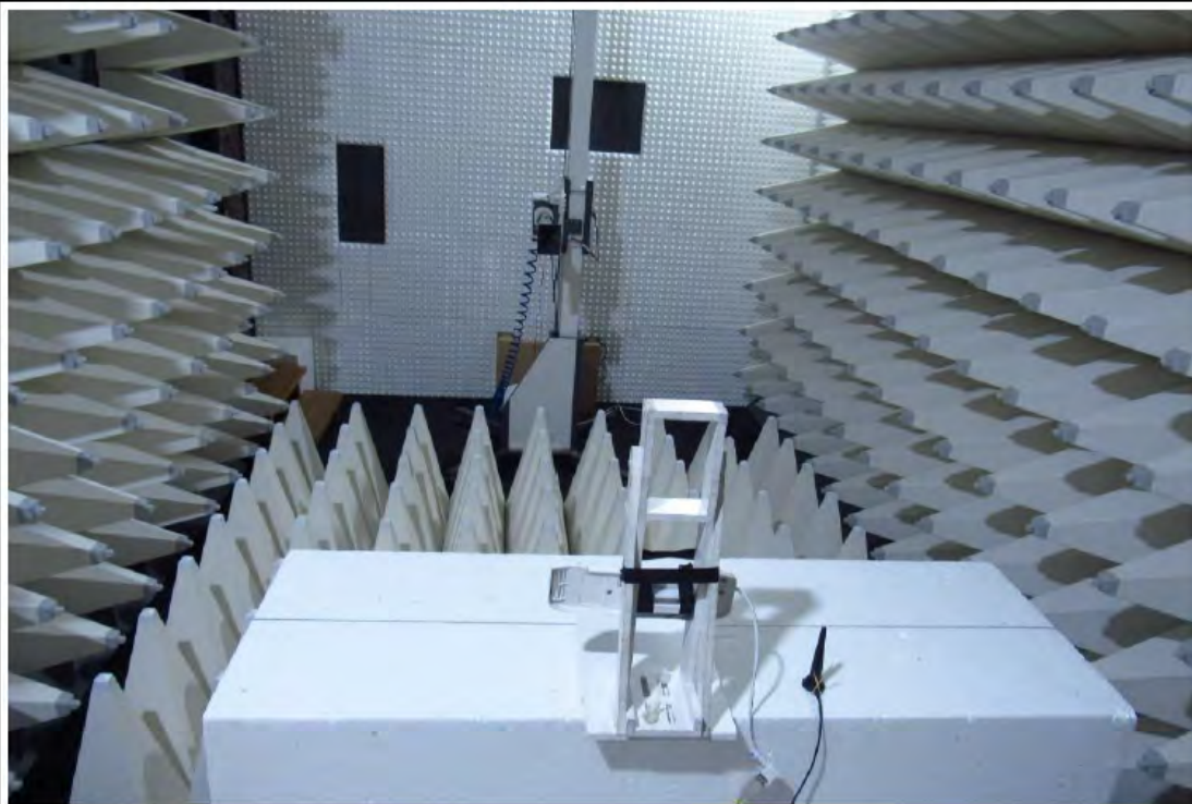
Setup 1 to 10 GHz
