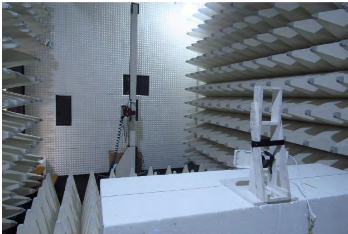
Setup 18 to 26.5 GHz A
