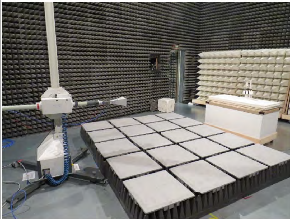
Setup 6.5 to 18 GHz
