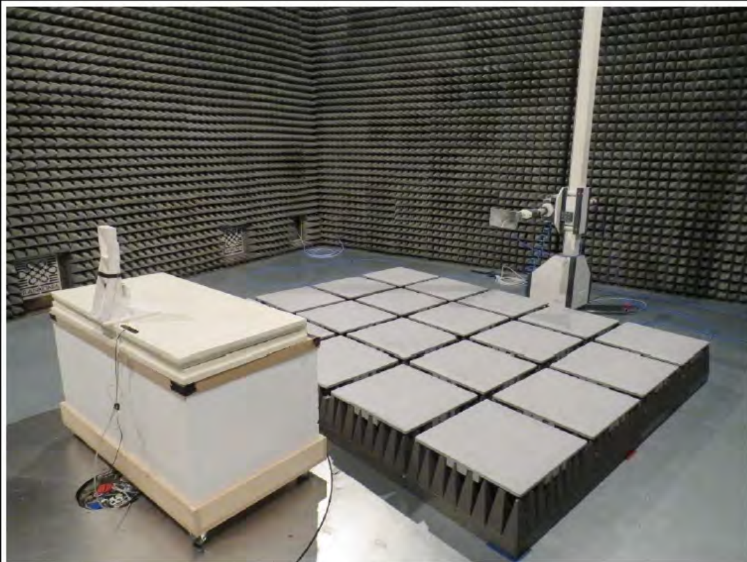
Setup 1 to 6.5 GHz
