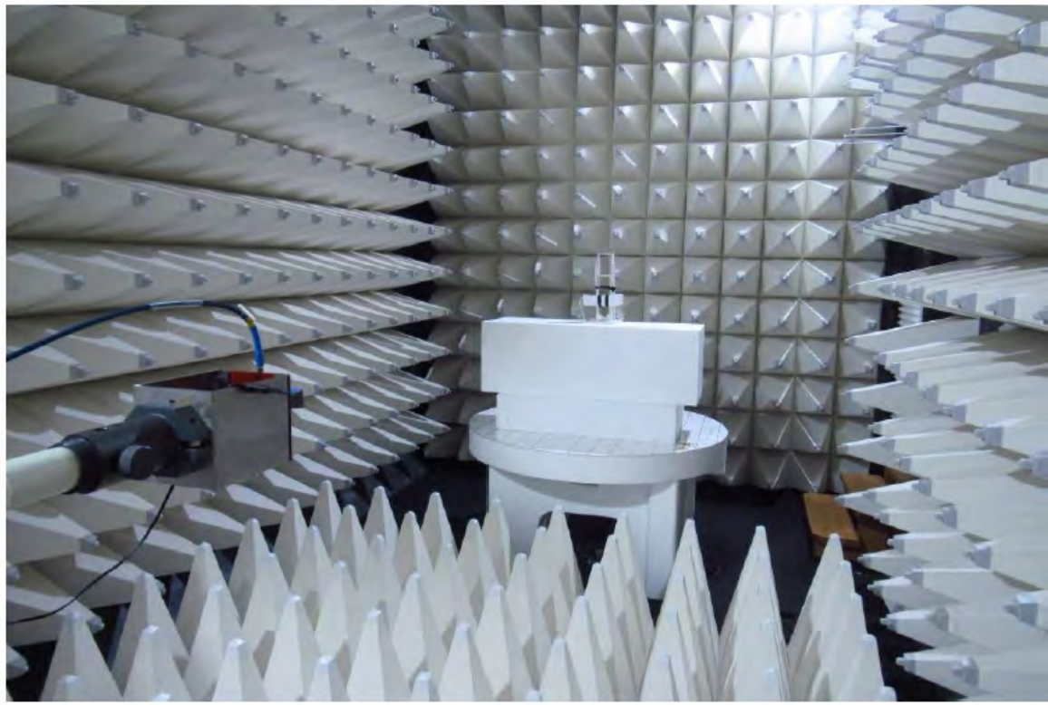
Setup 18 to 26.5 GHz B
