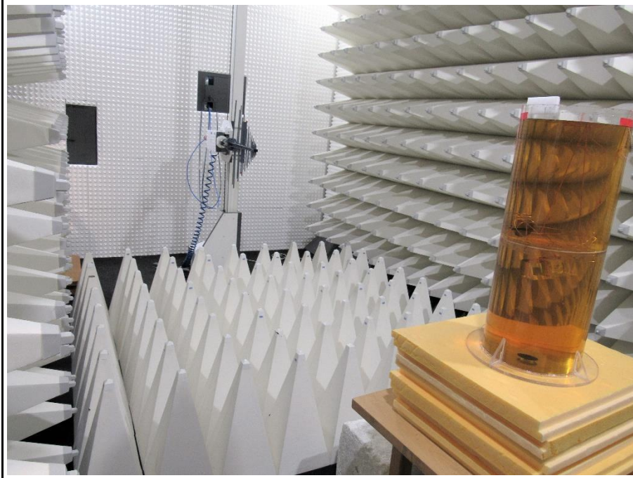
Test setup – Antenna pattern measurement
