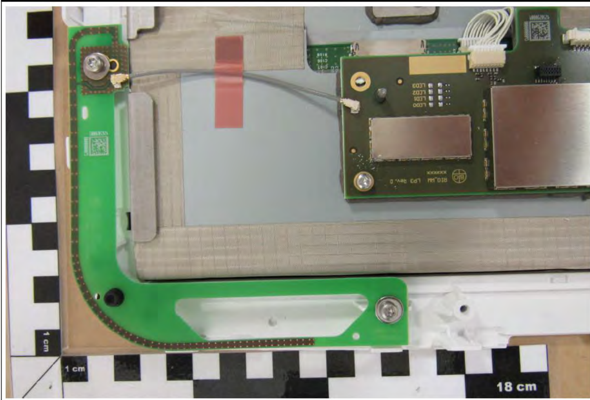
MICS-P Ant2
