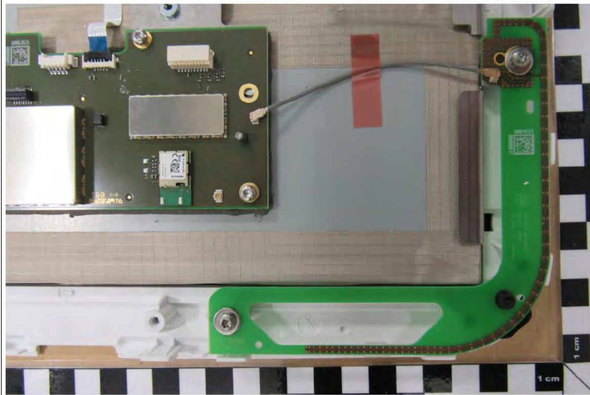
MICS-P Ant1
