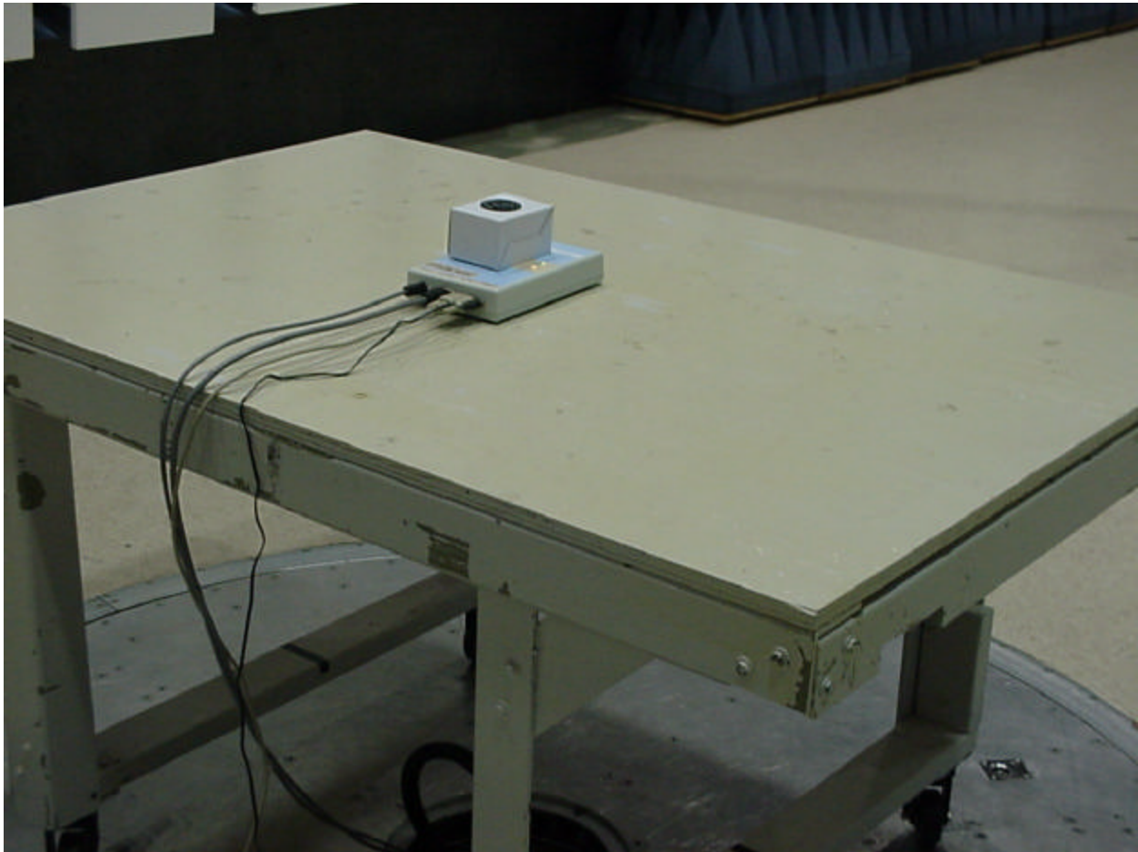
Figure 12 - Radiated Emissions Test Setup (Chamber - Back)
