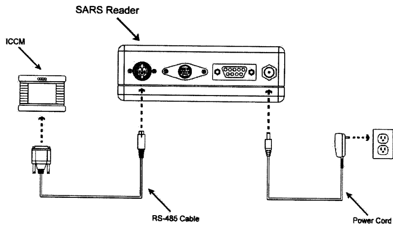
Figure 7: RS-485 Cable Installation
