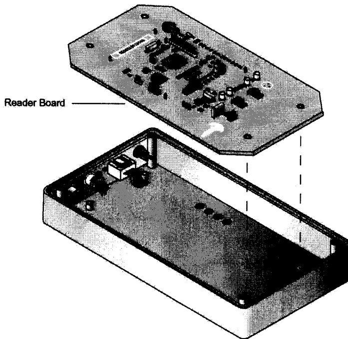
Figure 3: Reader Board and Enclosure
