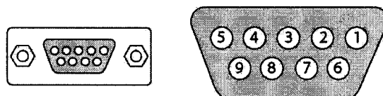
Figure 11: RS-232 Connector
