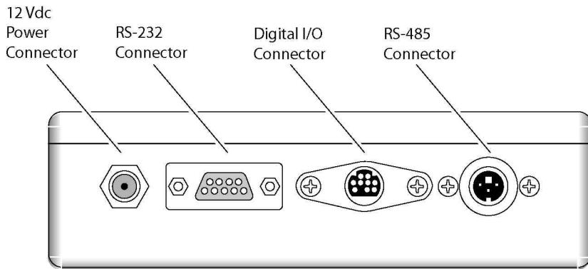
Figure 5: Reader End-Panel Connectors
