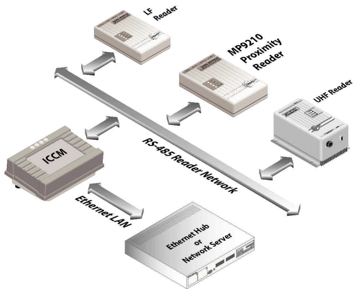
Figure 2: SAMSys Reader Network
