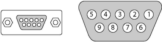
Figure 11: RS-232 Connector
