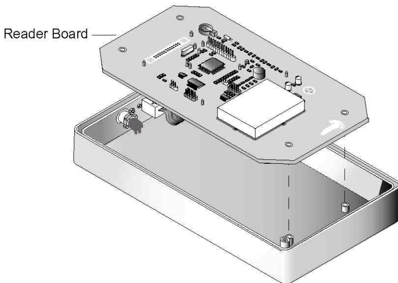
Figure 3: Reader Board and Enclosure
