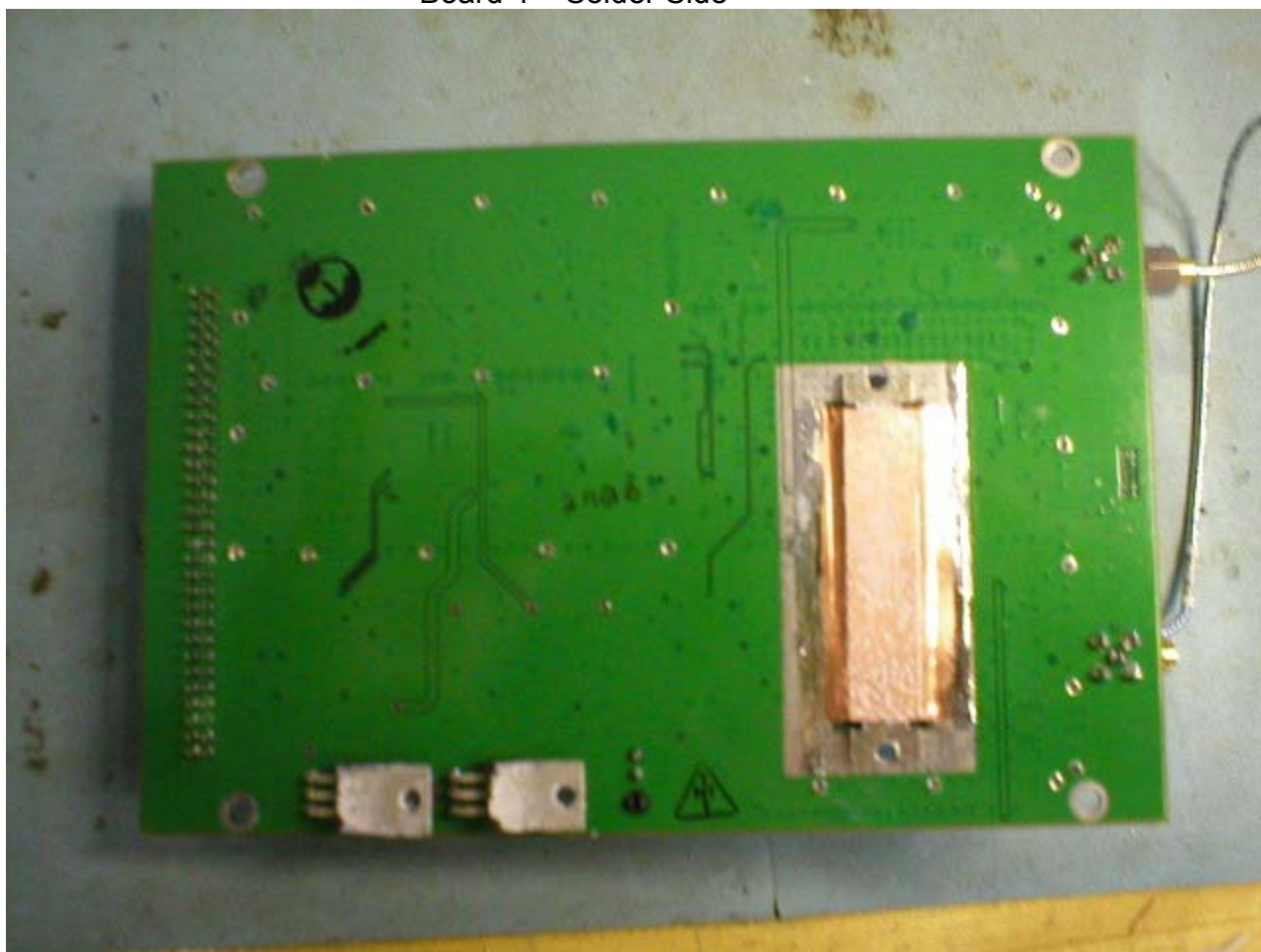
Board 4 – Solder Side
