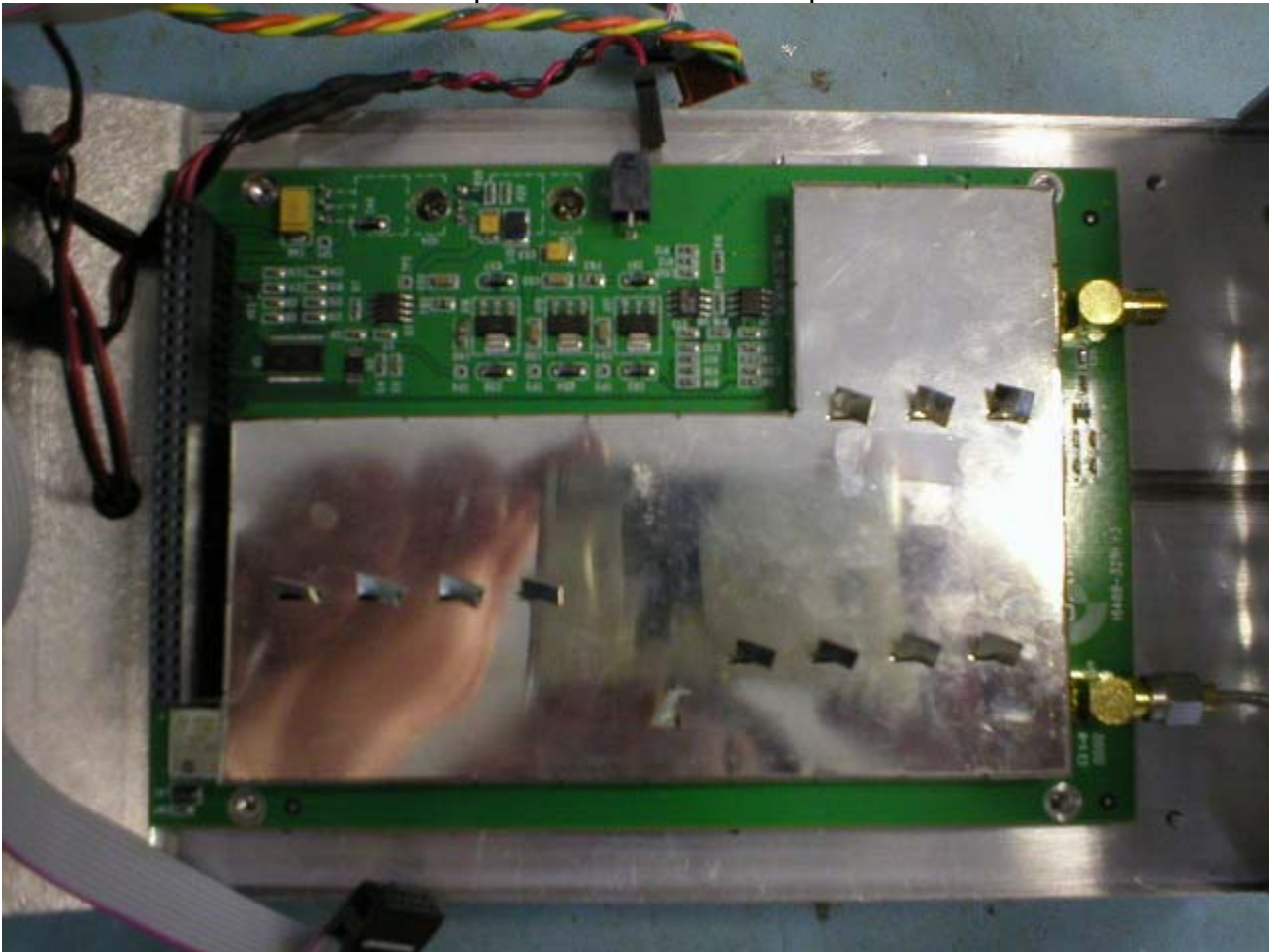
Board 4 – Component Side – Shield in place
