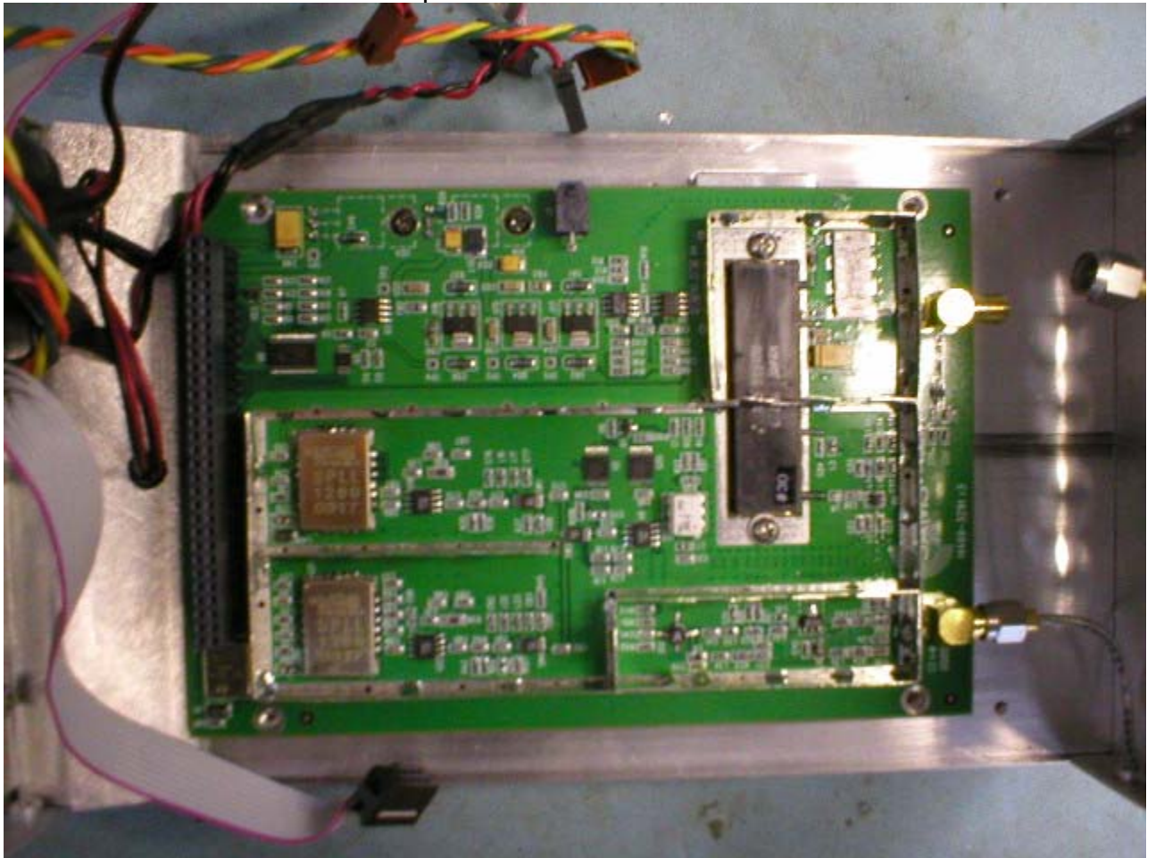
Board 4 – Component Side – Shield removed
