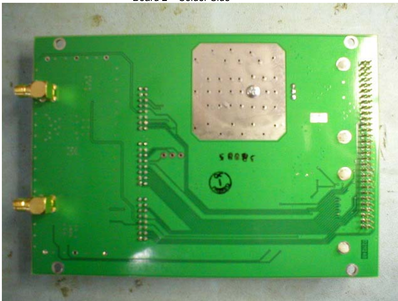
Board 2 – Solder Side
