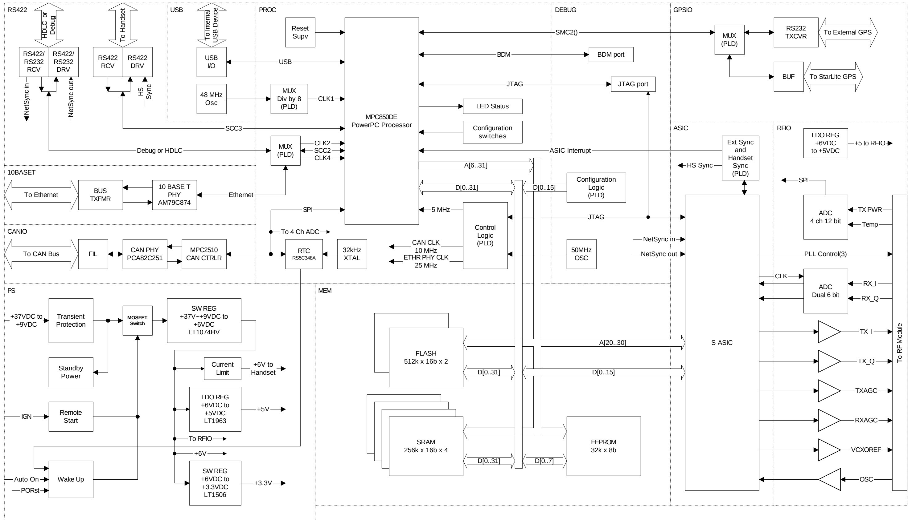
Spread Spectrum Radio Digital Block Diagram
