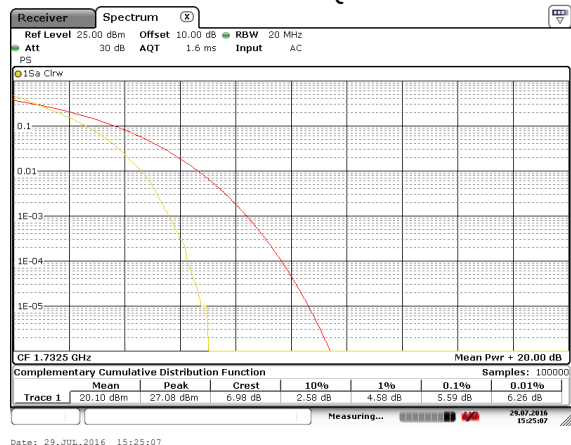
LTE Band 4 Middle channel
