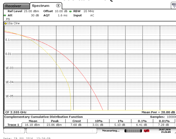
LTE Band 7 Middle channel
