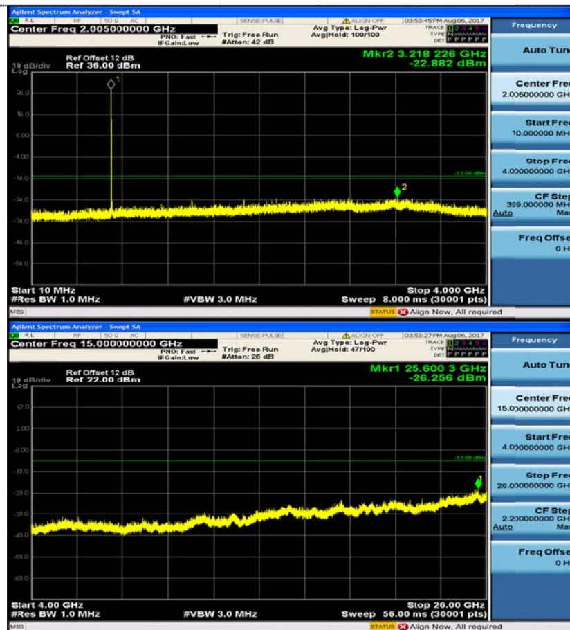
Channel High LTE Band 17-10MHz 16QAM
