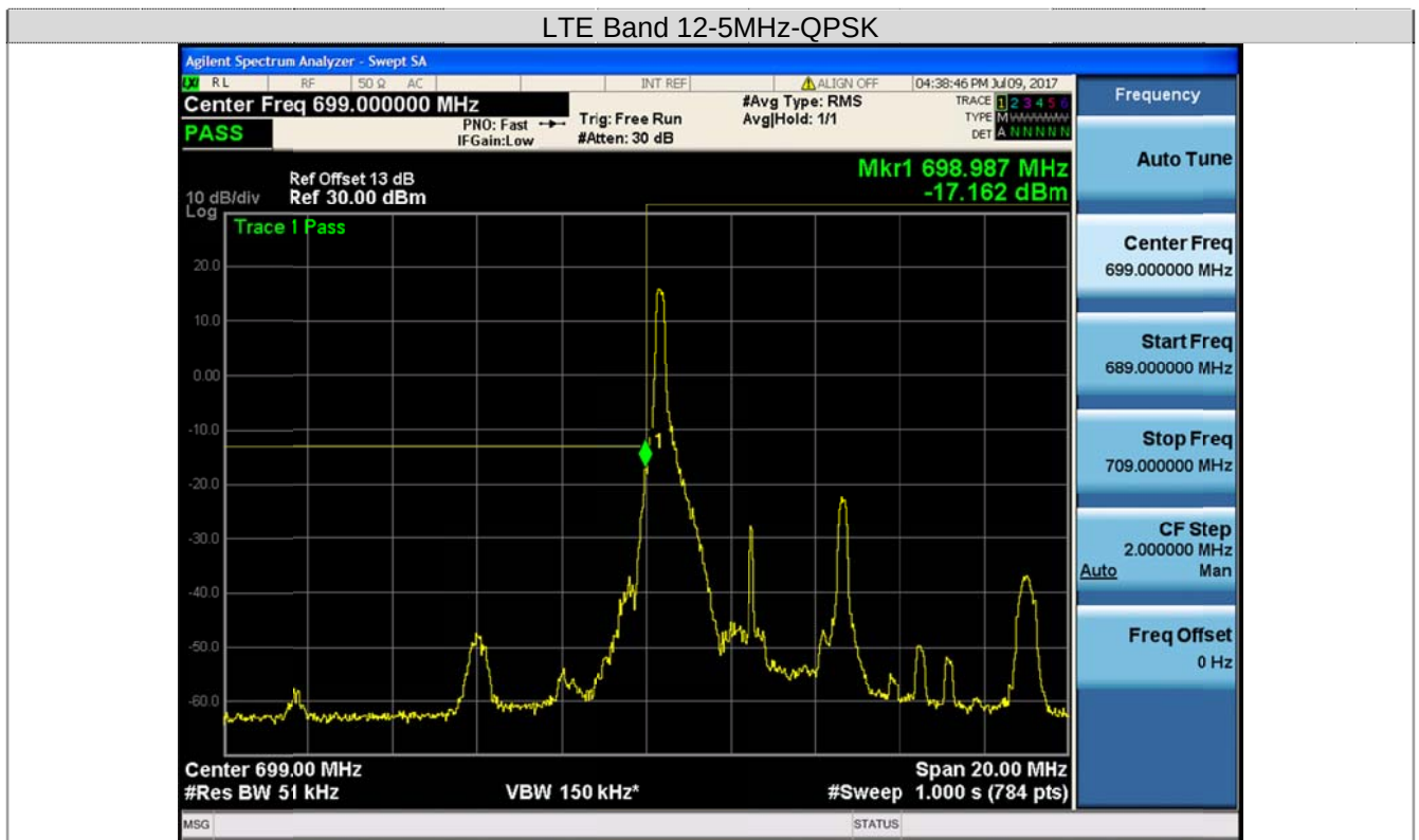
Channel Low-1RB#
