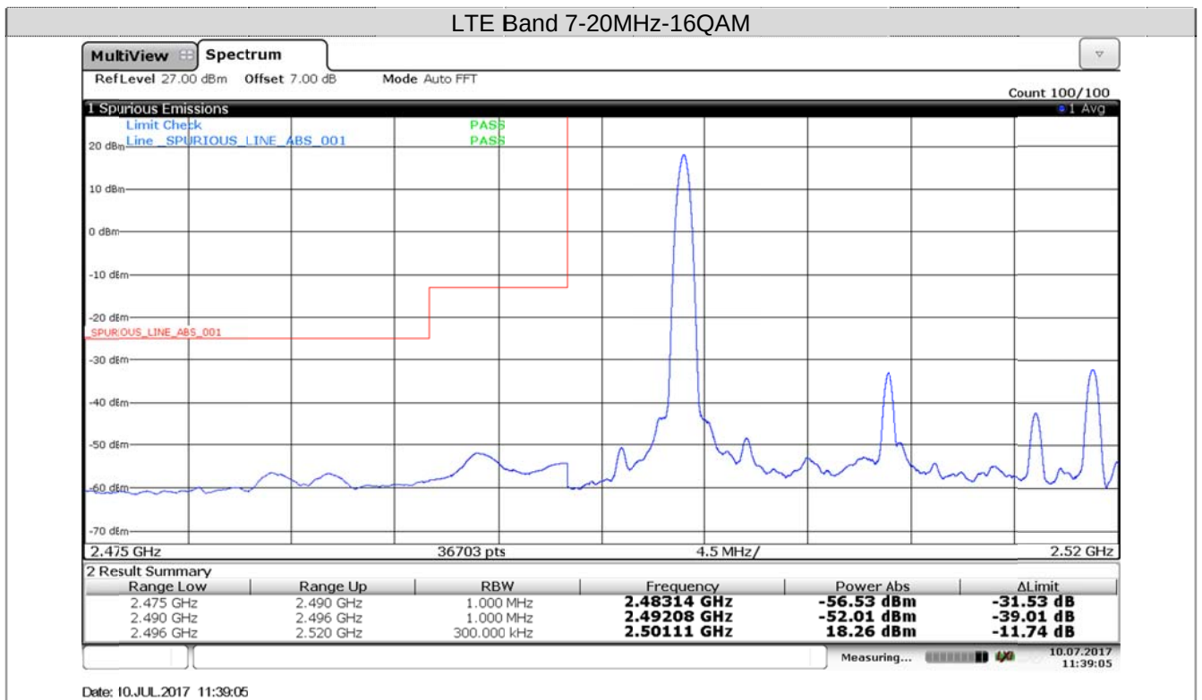
Channel Low-1RB#
