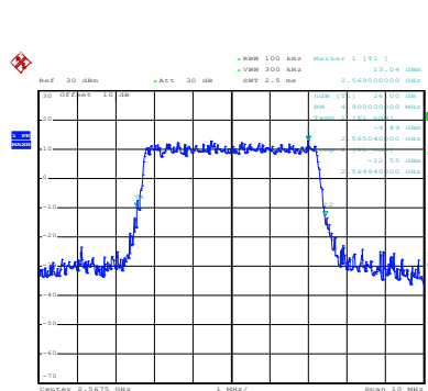
Modulation:16QAM
