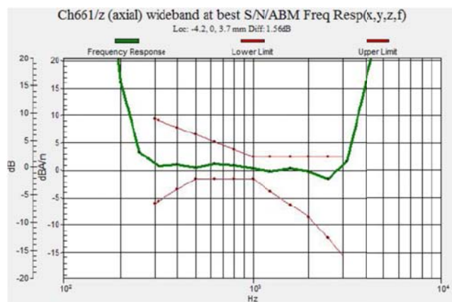
Fig 7.5 GSM1900 Ch661
