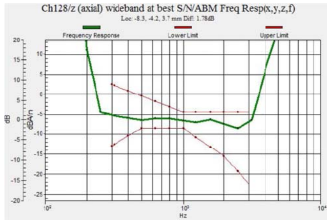
Fig 7.1 GSM850 Ch128
