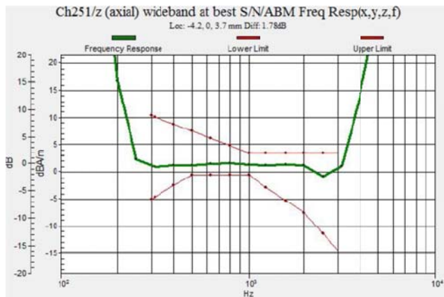
Fig 7.3 GSM850 Ch251
