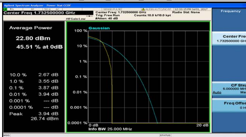
Band4_5MHz_QPSK_20175_1RB#0
