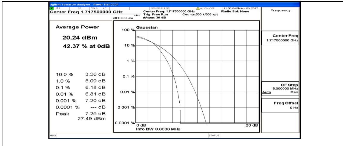
(Channel Bandwidth:15 MHz)_MCH_16QAM_1RB#0
