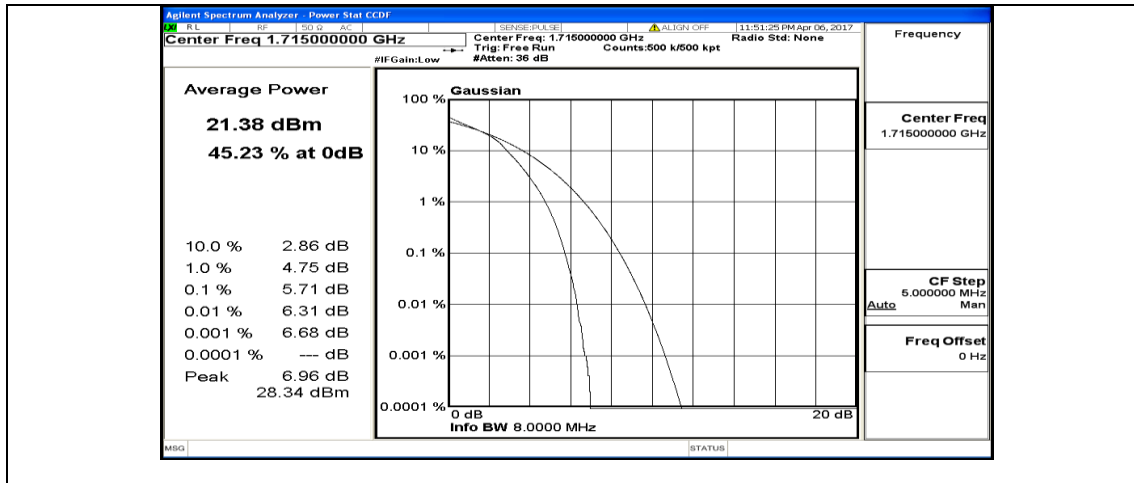
Channel Bandwidth: 10 MHz_MCH_16QAM_1RB#0
