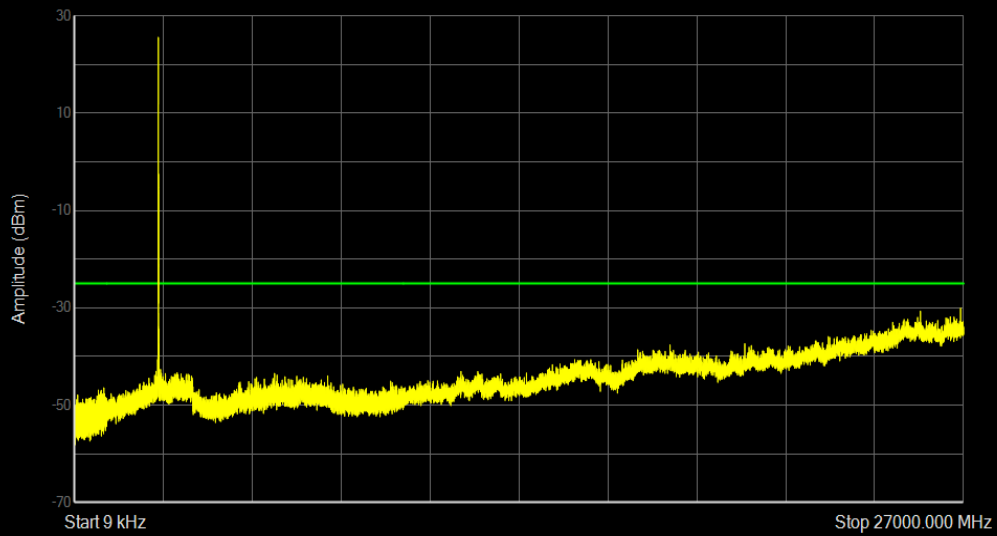
Band7 16QAM BW=10MHz Channel=21400 RB Size=1 Position=#0
