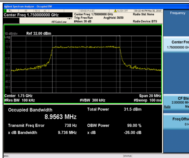
Band4_10MHz_QPSK_17500_50RB#0
