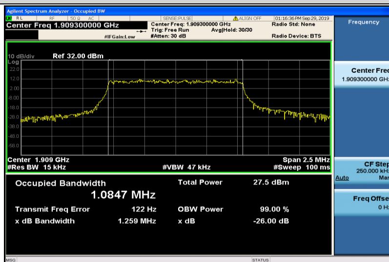
Band2-1.4MHz-QPSK-19193-6RB#0-1.0847
