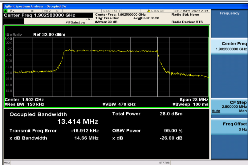
Band2-15MHz-16QAM-19125-75RB#0-13.414
