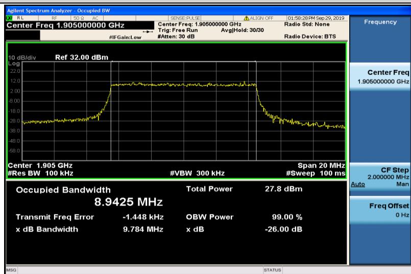
Band2-10MHz-16QAM-19150-50RB#0-8.9425
