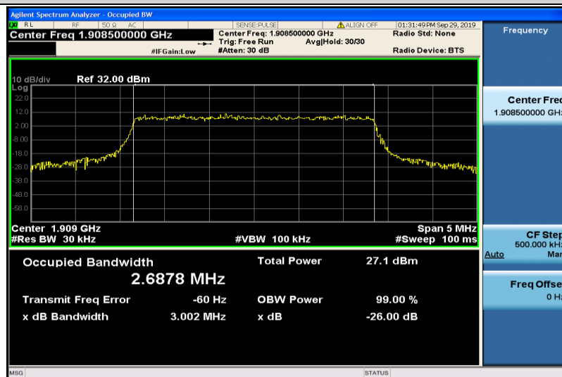
Band2-3MHz-16QAM-19185-15RB#0-2.6878
