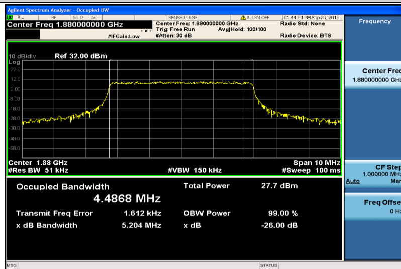
Band2-5MHz-16QAM-18900-25RB#0-4.4868
