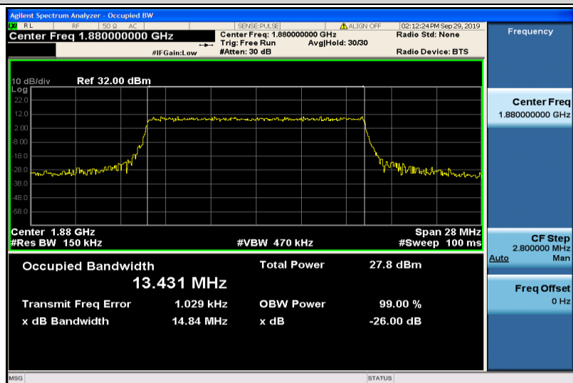
Band2-15MHz-16QAM-18900-75RB#0-13.431
