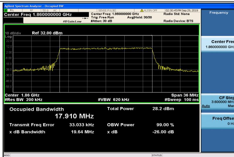
Band2-20MHz-16QAM-18700-100RB#0-17.910
