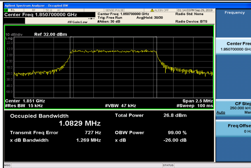
Band2-1.4MHz-16QAM-18607-6RB#0-1.0829
