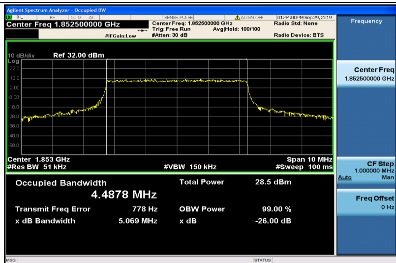
Band2-5MHz-QPSK-18625-25RB#0-4.4878
