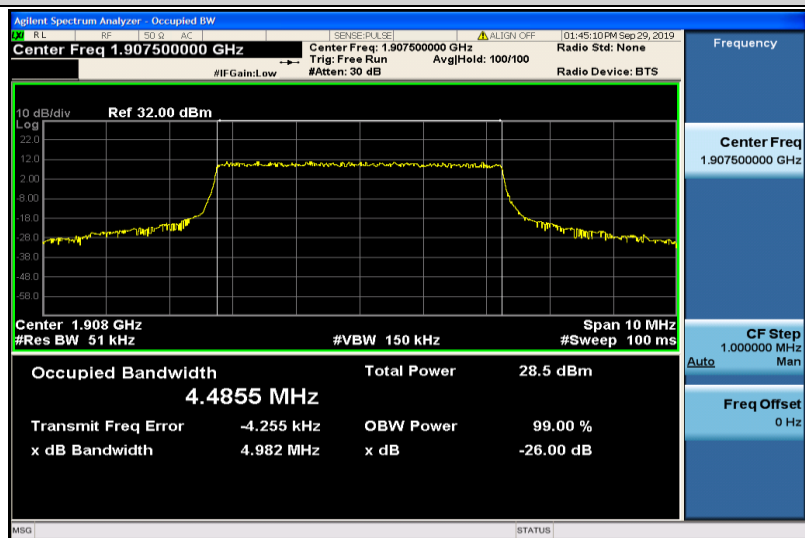
Band2-5MHz-QPSK-19175-25RB#0-4.4855
