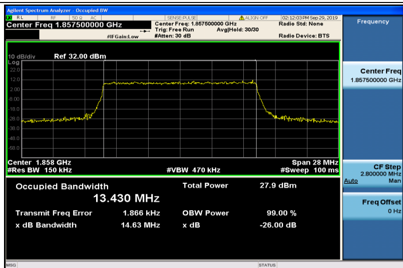
Band2-15MHz-16QAM-18675-75RB#0-13.430
