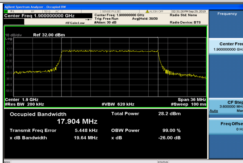
Band2-20MHz-16QAM-19100-100RB#0-17.904
