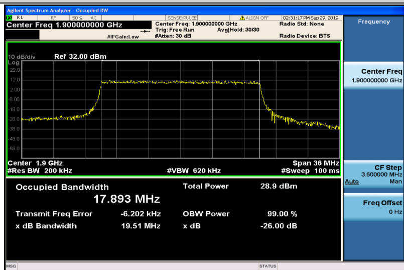
Band2-20MHz-QPSK-19100-100RB#0-17.893
