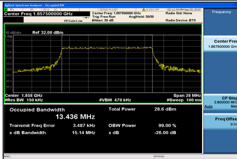
Band2-15MHz-QPSK-18675-75RB#0-13.436
