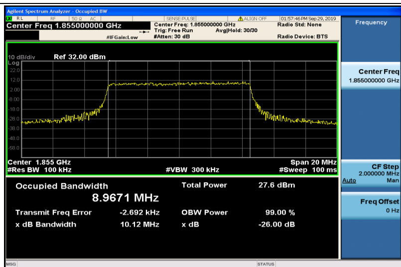
Band2-10MHz-16QAM-18650-50RB#0-8.9671
