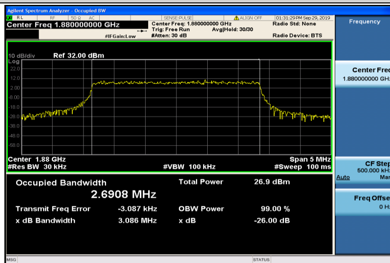
Band2-3MHz-16QAM-18900-15RB#0-2.6908
