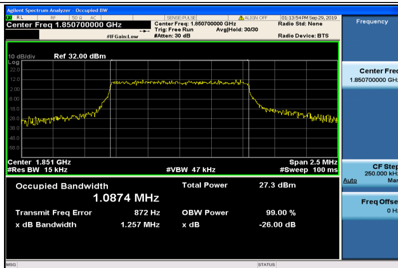
Band2-1.4MHz-QPSK-18607-6RB#0-1.0874
