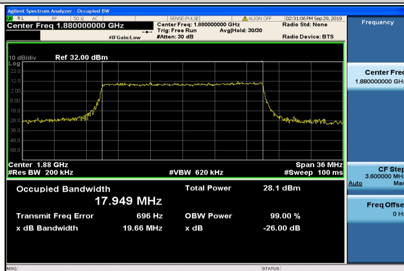
Band2-20MHz-16QAM-18900-100RB#0-17.949
