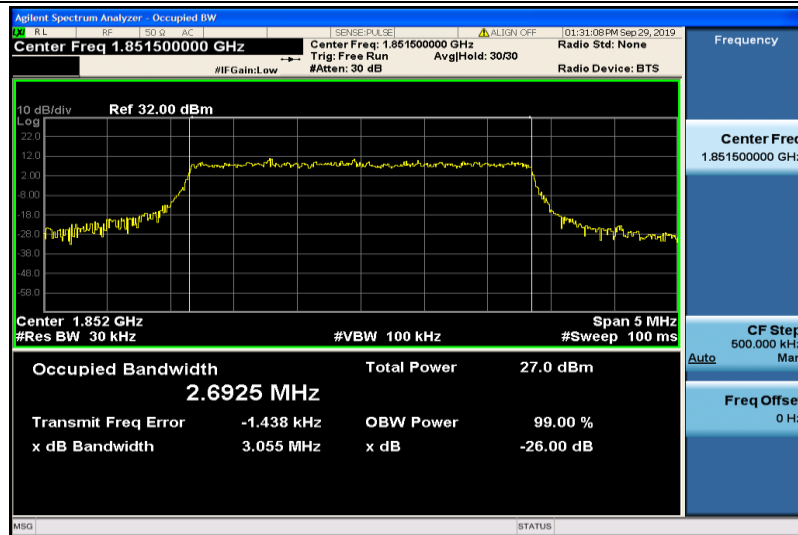
Band2-3MHz-16QAM-18615-15RB#0-2.6925
