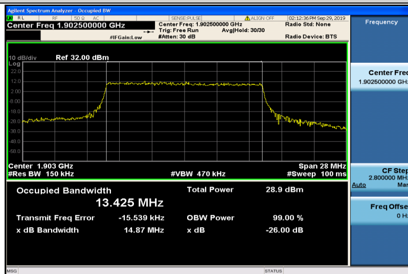
Band2-15MHz-QPSK-19125-75RB#0-13.425
