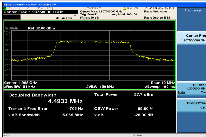
Band2-5MHz-16QAM-19175-25RB#0-4.4933
