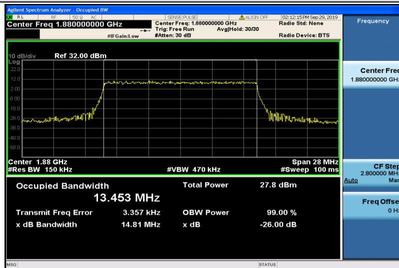
Band2-15MHz-QPSK-18900-75RB#0-13.453
