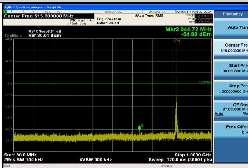
Band5-1.4MHz-QPSK-20407-1RB#0-30~1000MHz
