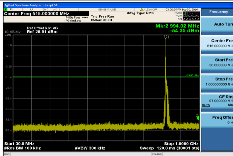
Band5-10MHz-16QAM-20450-1RB#0-30~1000MHz
