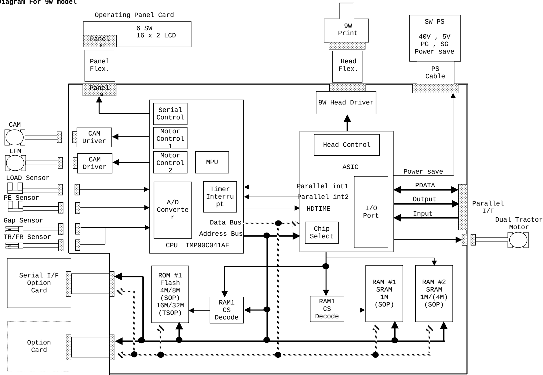
Block Diagram For 9W model
