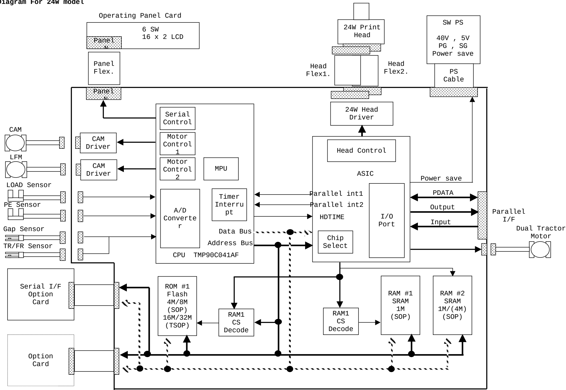
Block Diagram For 24W model
