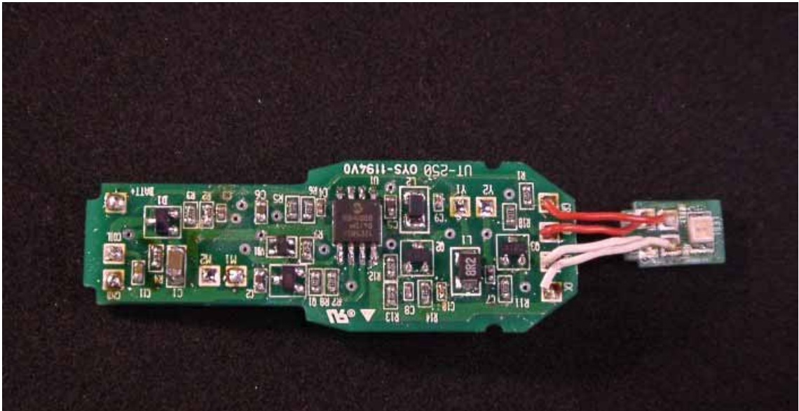
Internal Photo 5: PC Board, component side
