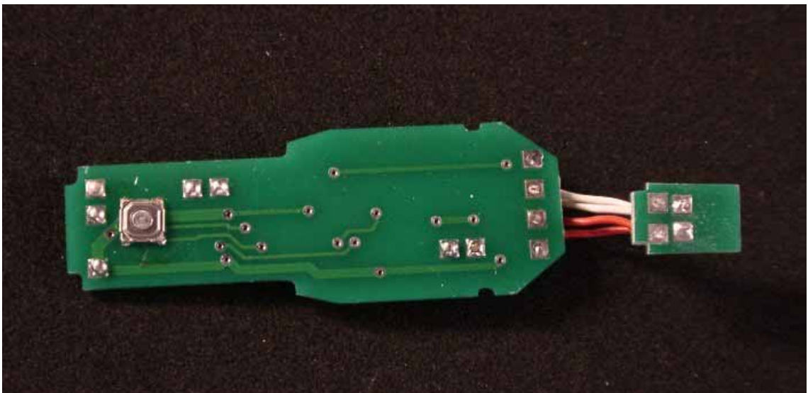
Internal Photo 6: PC Board, foil side
