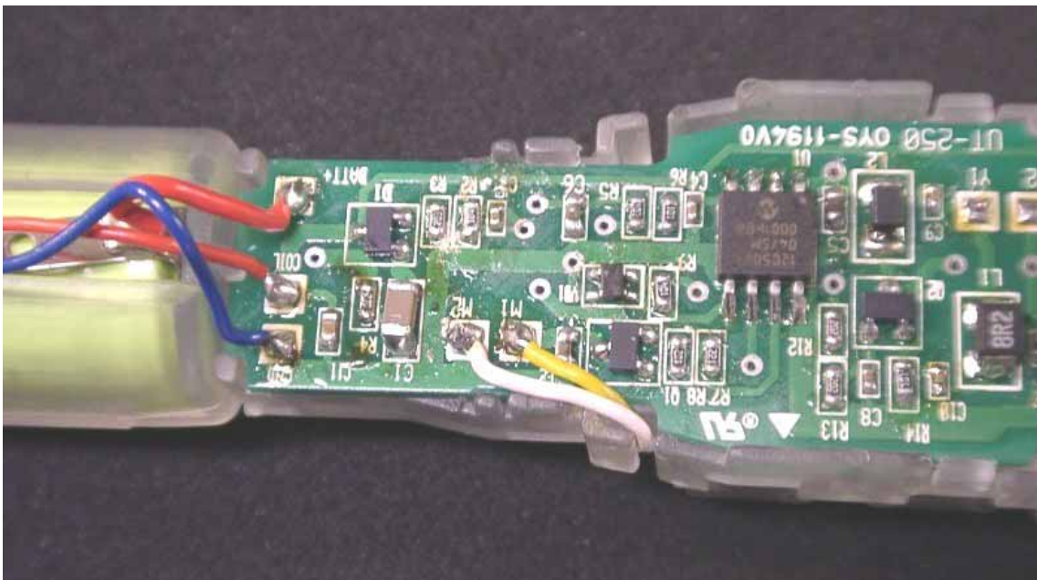
Internal Photo 4: Zoom-up of PC Board
