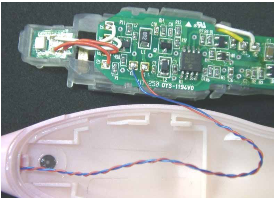
Internal Photo 2: Zoom-up inside of the tooth brush
