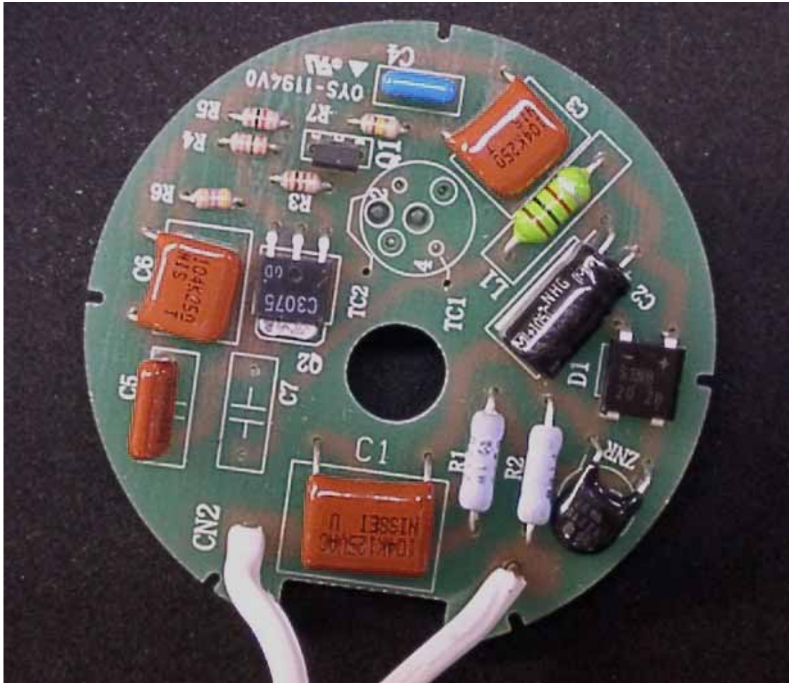
Internal Photo 7: The Board of Changer, Component Side
