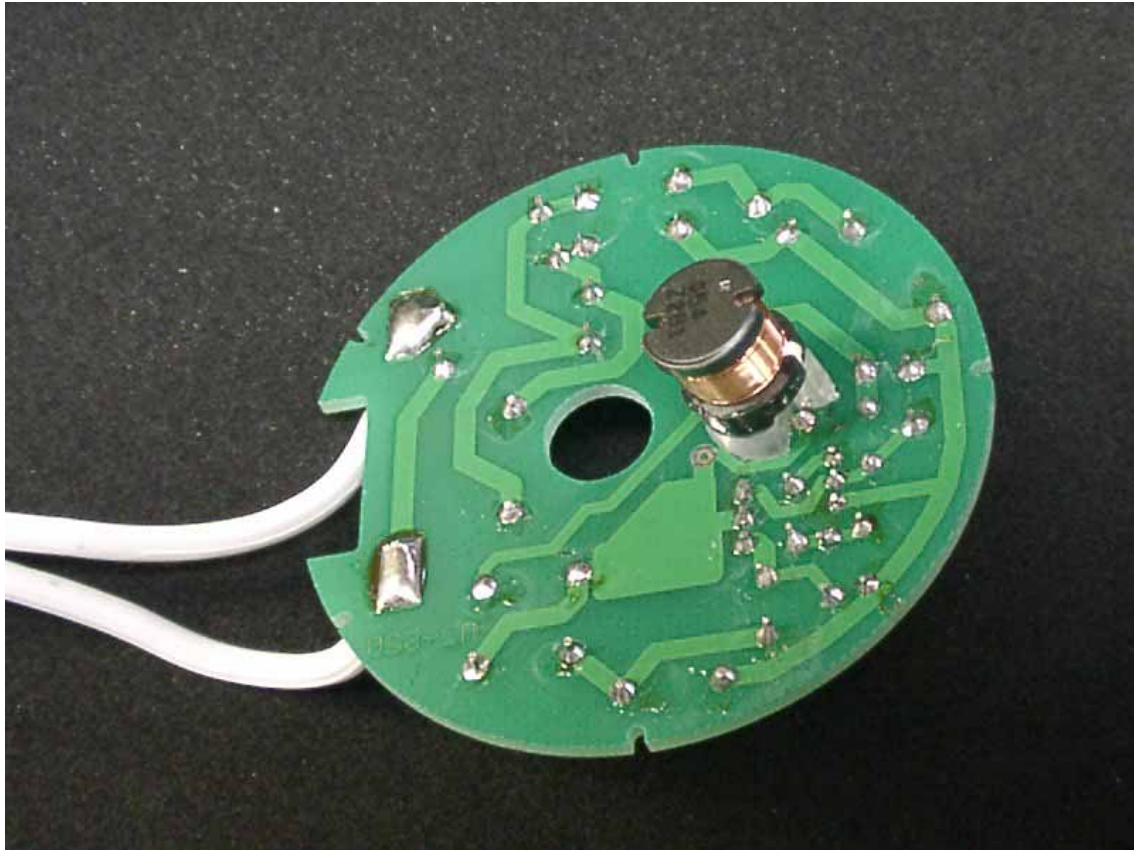
Internal Photo 8: The board of charger, Foil Side
