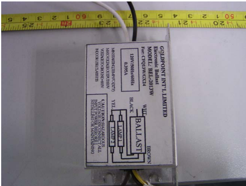
DW005 - Inside View (1)
