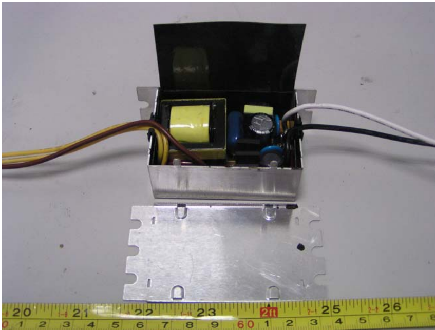
DW005 -PCB View (1)
