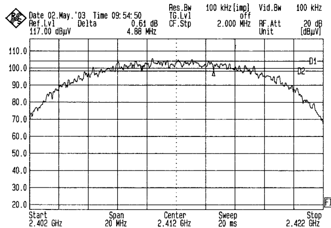
Channel 1
