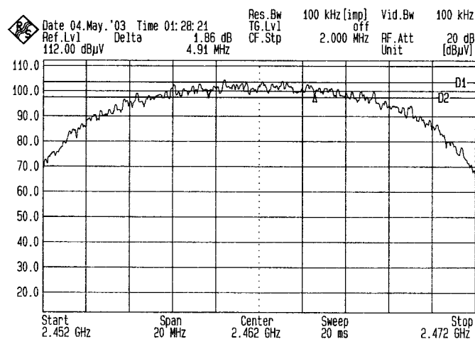
Channel 11
