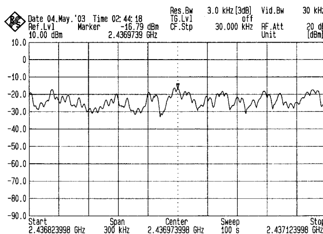
Channel 6
