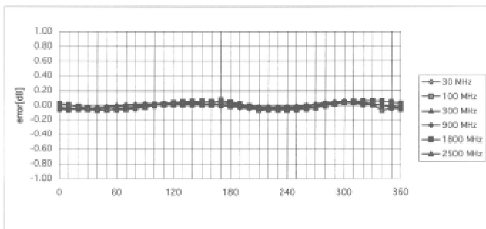
Isotropy Error ( \phi ), \theta = 0^\circ
