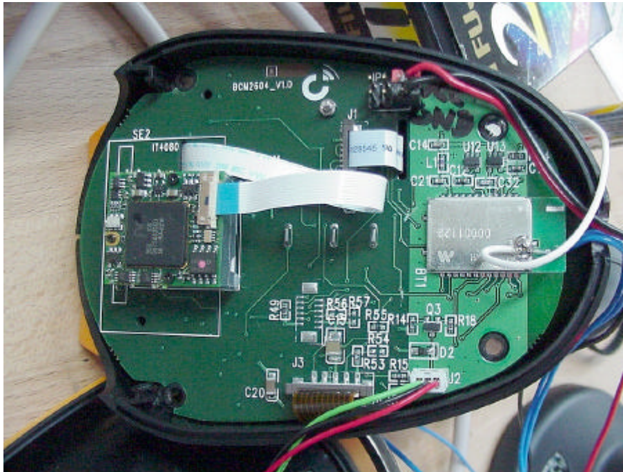
Picture 2 : EUT inside view (with temporary antenna connector on the right side)
