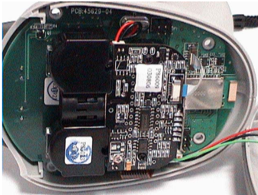
Board with CCD scan engine (BC2604)
