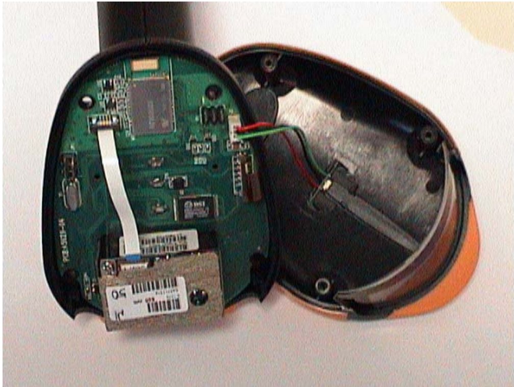
Board with Laser scan engine (BL2604)
