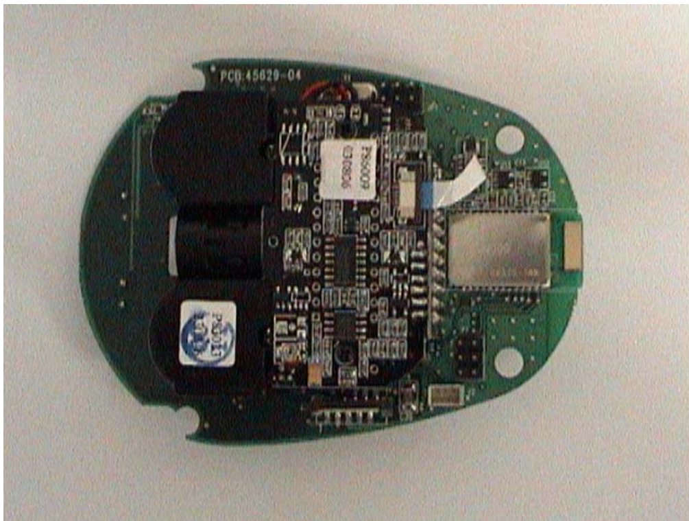
Board with CCD scan engine (BC2604)
