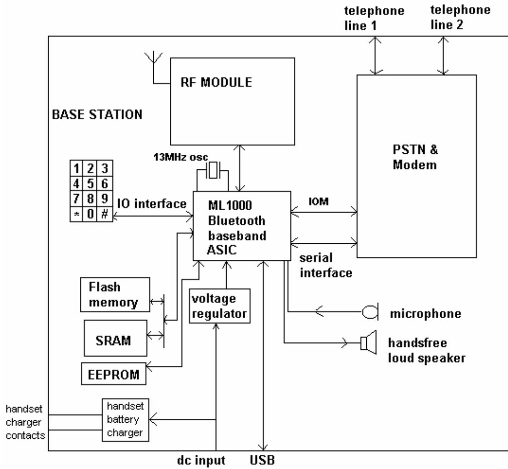
BASE STATION Block Diagram
