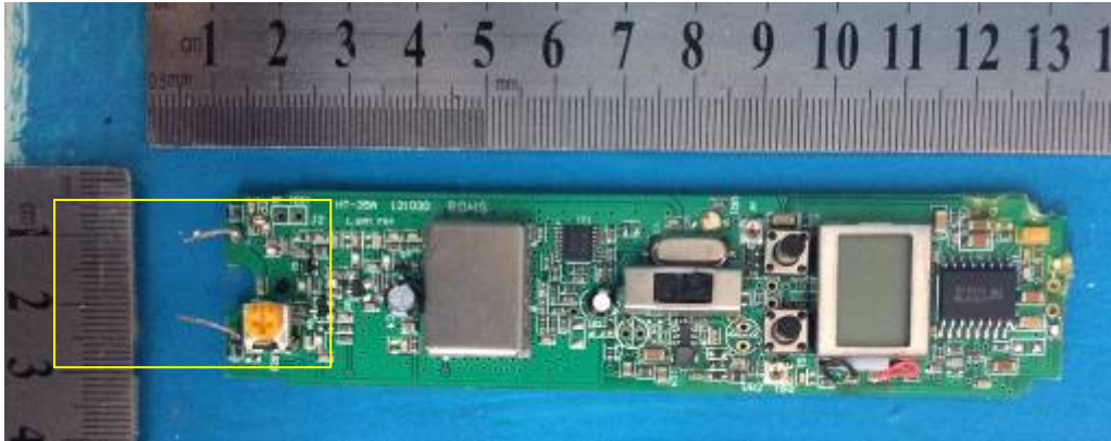
HT-35A Antenna: Batteries return circuit
