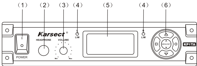
Front panel
