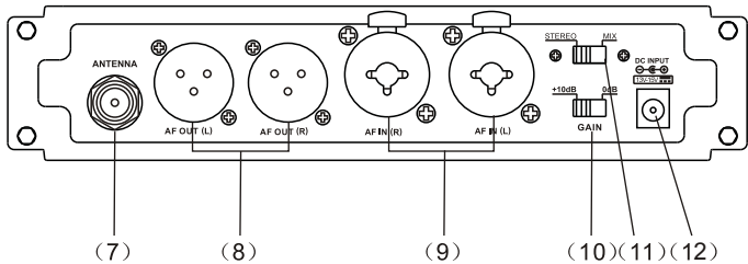
Rear panel
