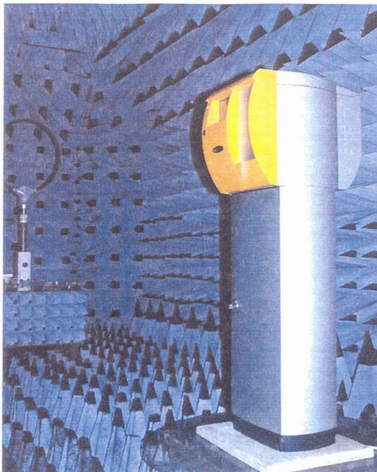
Photo No. 1, Park Column AS 450 SA00-BLL in the full anechoic chamber.
