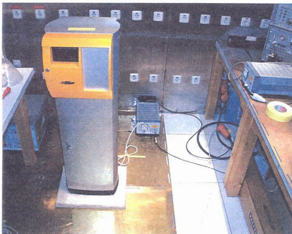
Photo No. 2, Park Column AS 450 SA00-BLL at the conducted emissions measurement place.
