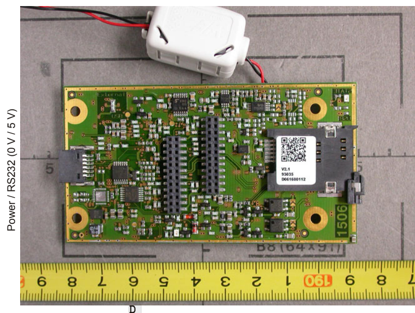
Fig. 2: rear view sd705
