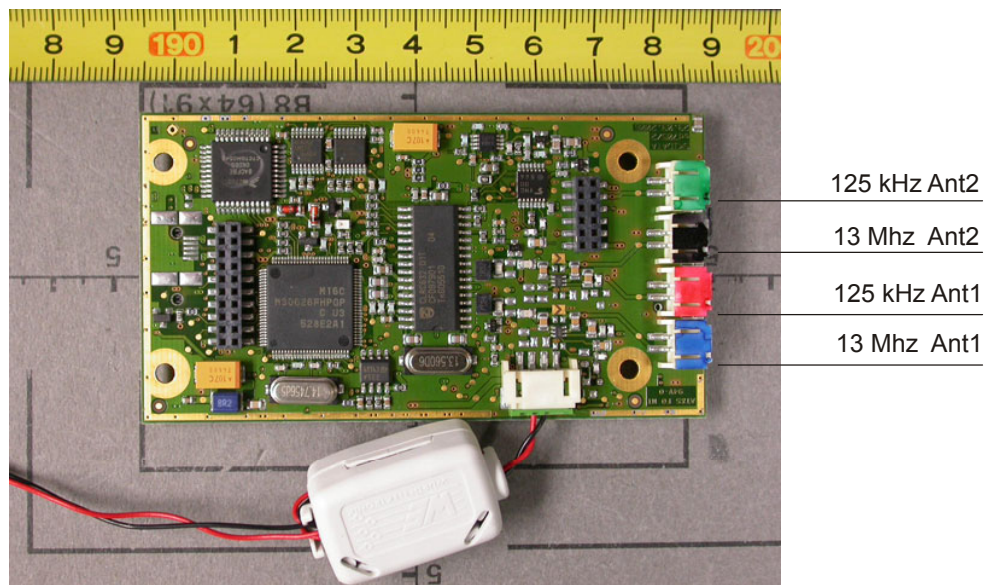
Fig. 1: front view sd705
